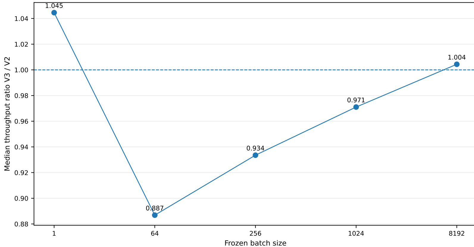
Stage26-4C3 paired implementation sensitivity
