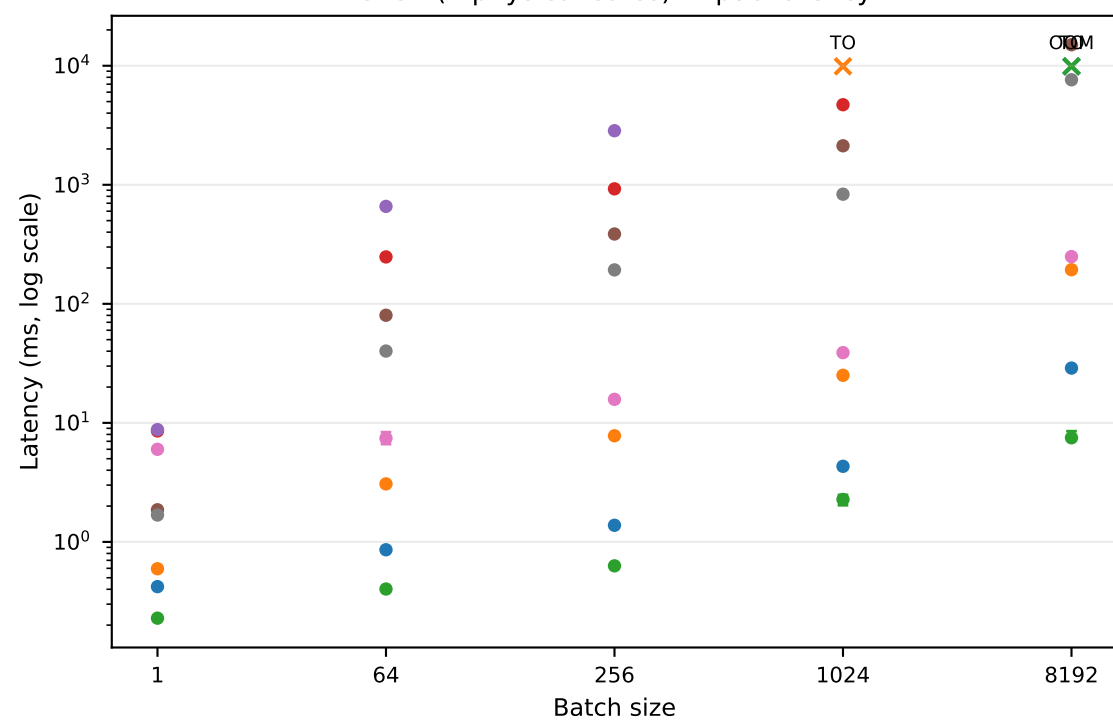
CPU2 (2 physical cores) — p50 latency
