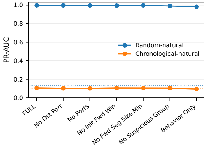
(a) PR-AUC
