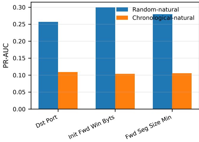
(a) Single-feature PR-AUC
