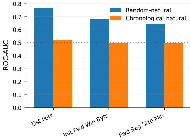
(b) Single-feature ROC-AUC
