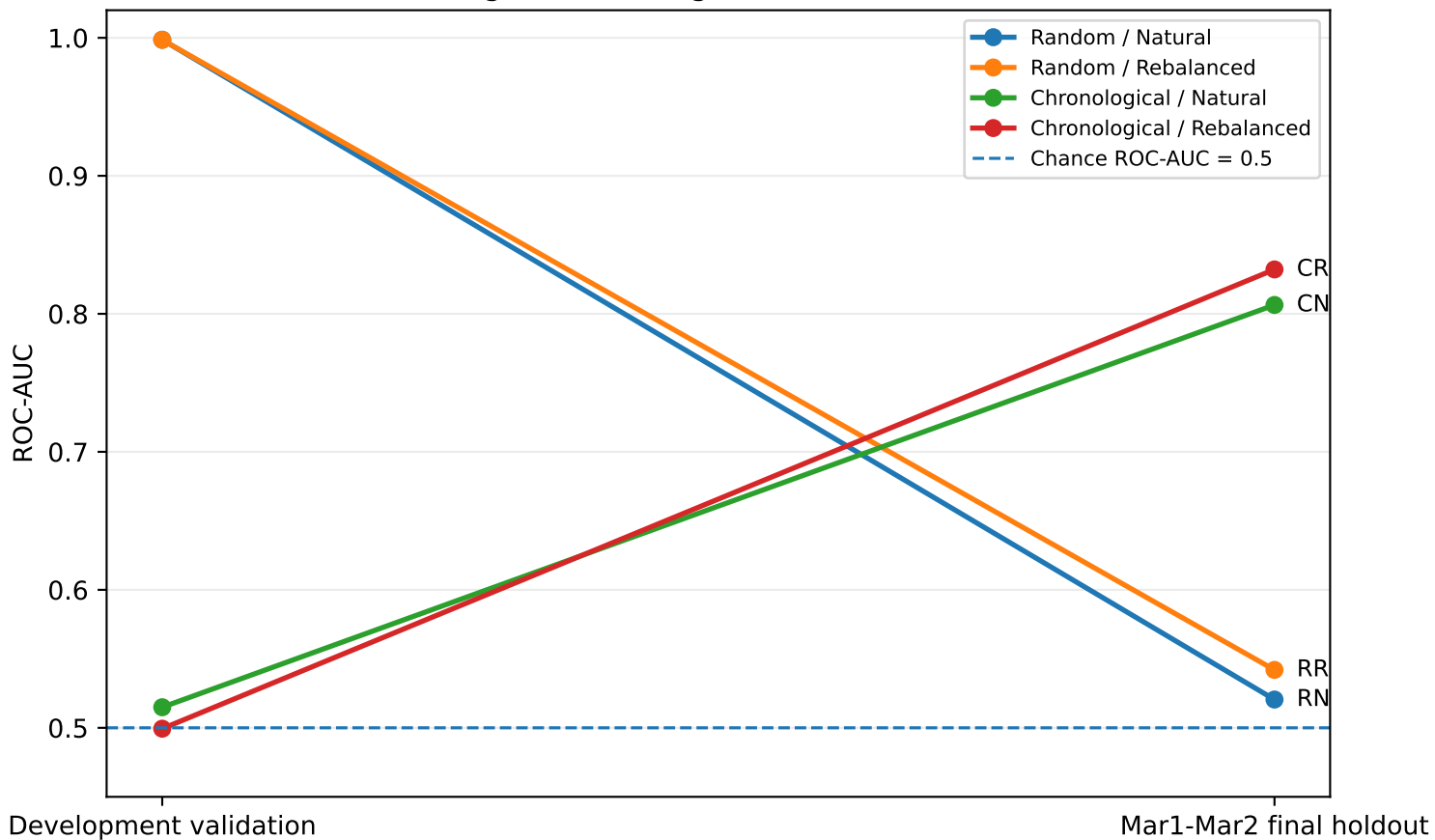
Stage22R ranking transfer: ROC-AUC
