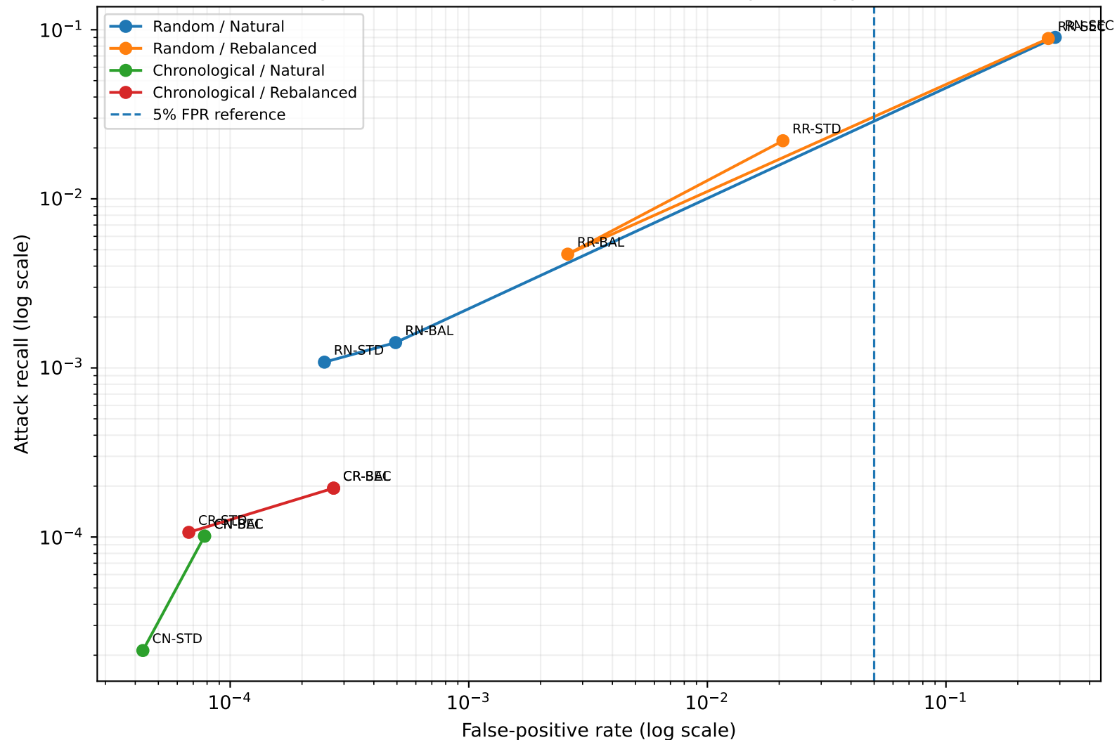
Stage22R final behavior at all 12 frozen operating points
