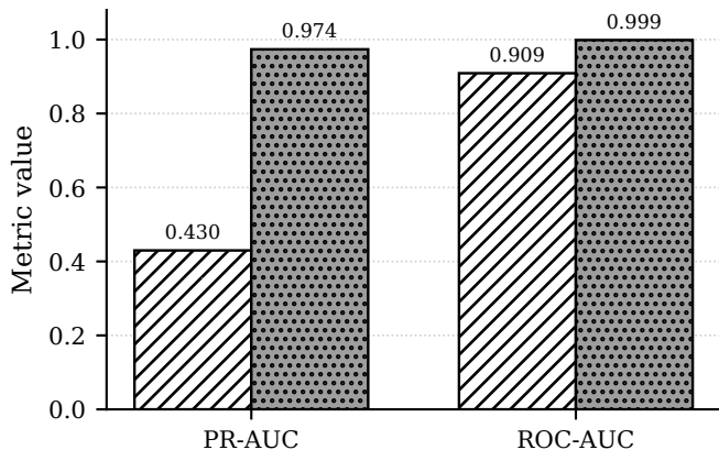
(a) Threshold-free ranking
