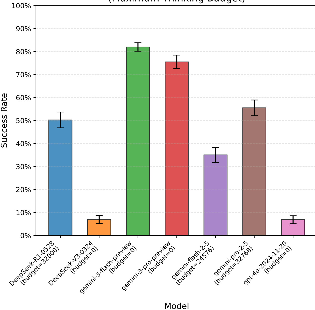
Success Rate Across All Models (Maximum Thinking Budget)
