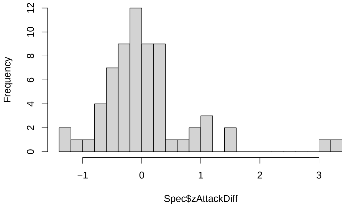
Histogram of Spec$zAttackDiff
