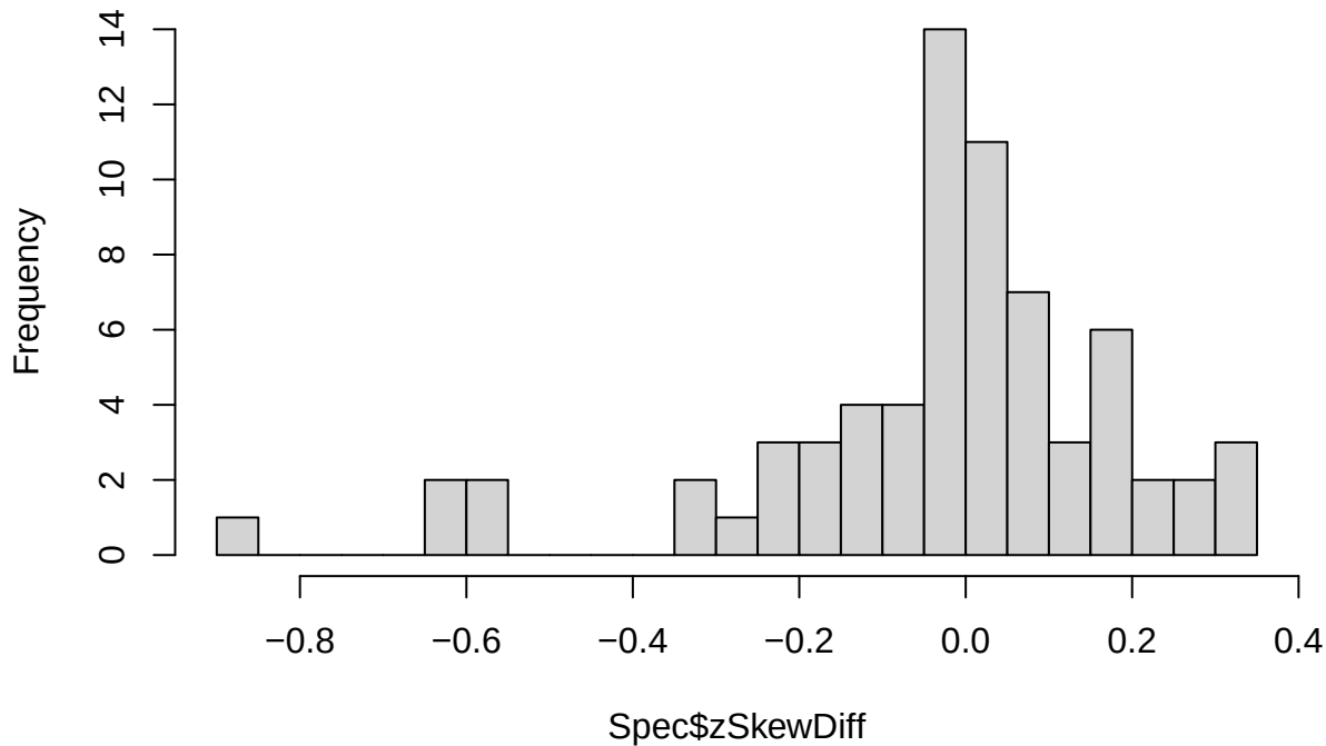
Histogram of Spec$zSkewDiff
