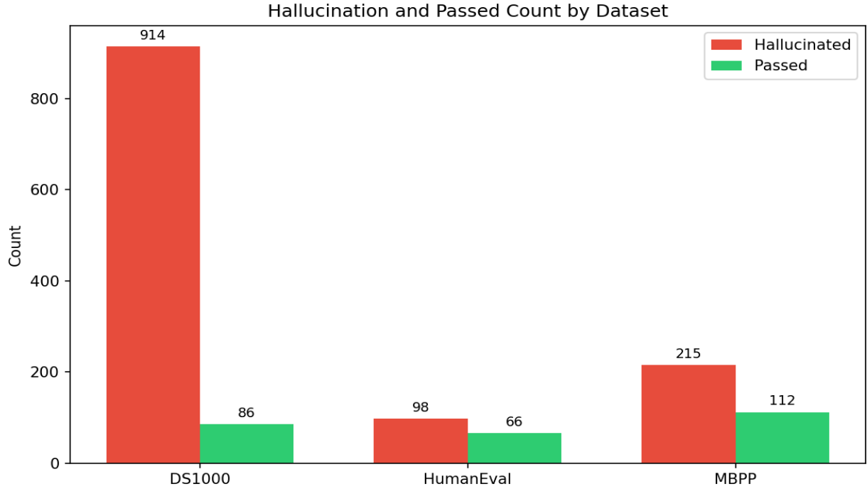
Fig 5.1 Hallucination Vs Passed count across dataset
