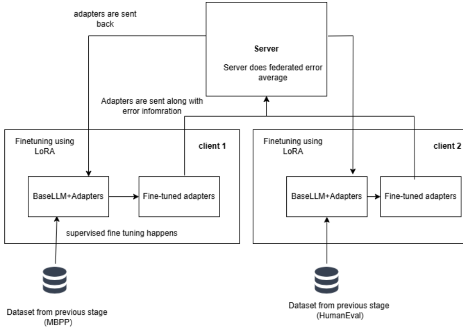
Figure: 3.2 LoRA Fine tuning and federated aggregation
