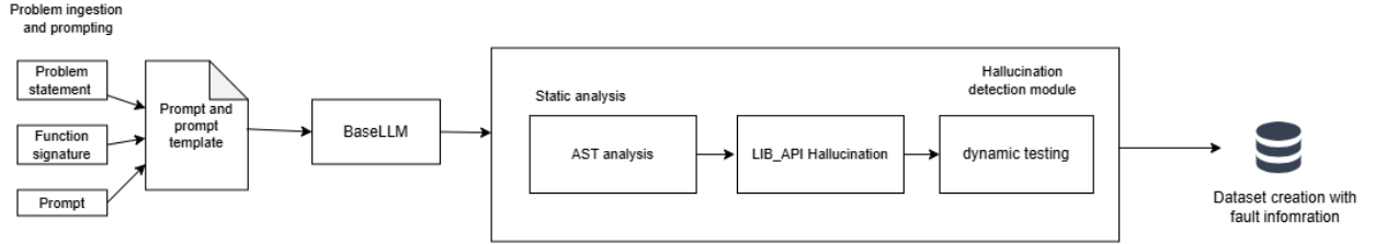
Figure: 3.1 – Client-side hallucination detection and dataset construction framework
