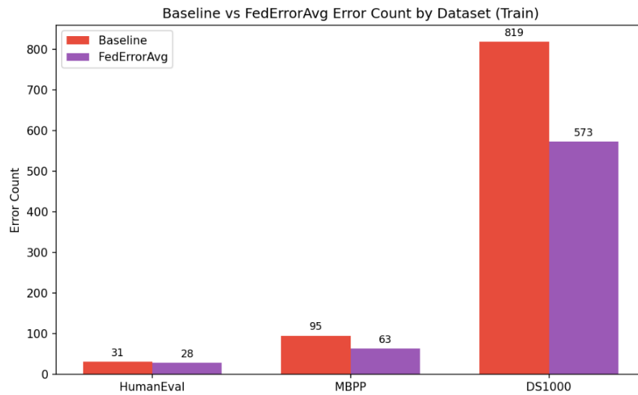
Fig 5.4 Hallucination count(Baseline Vs FedErrorAvg)
