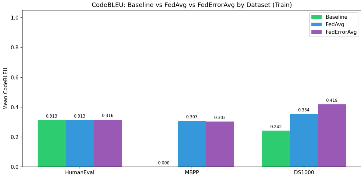
Fig 5.8 CodeBLEU comparison between baseline, FedAvg and FedErrorAvg
