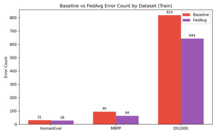
Fig 5.2 Hallucination count(Baseline Vs FedAvg
