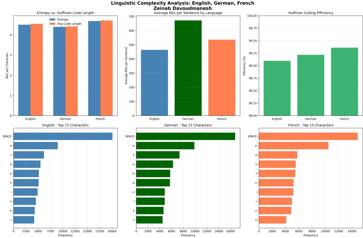
Figure 1: Comprehensive analysis of linguistic complexity across English, German, and French. Top row: (left) entropy vs. code length comparison, (center) average bits per sentence, (right) Huffman coding efficiency. Bottom row: character frequency distributions for each language.
