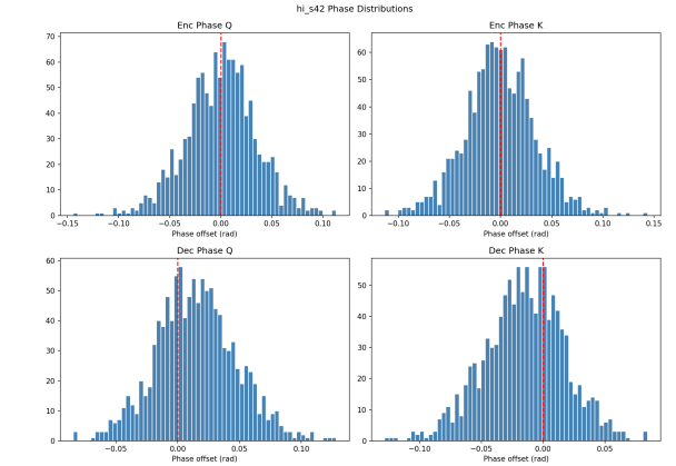
Fig. 3. Hi-En phase distributions. Dashed line: zero (RoPE init).
