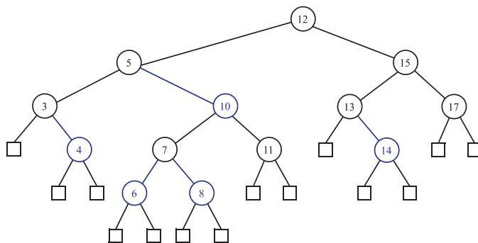
Figure 10.27: Red-black tree associated with the (2,4) tree of Figure 10.21. Each external node of this red-black tree has 4 black ancestors (including itself); hence, it has black depth 3. We use the color blue instead of red. Also, we use the convention of giving an edge of the tree the same color as the child node.
