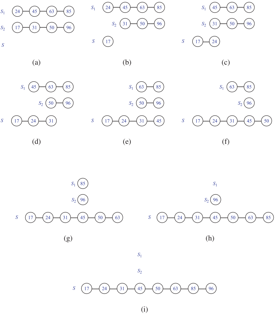
Figure 11.6: An execution of the algorithm merge shown in Code Fragment 11.2.
