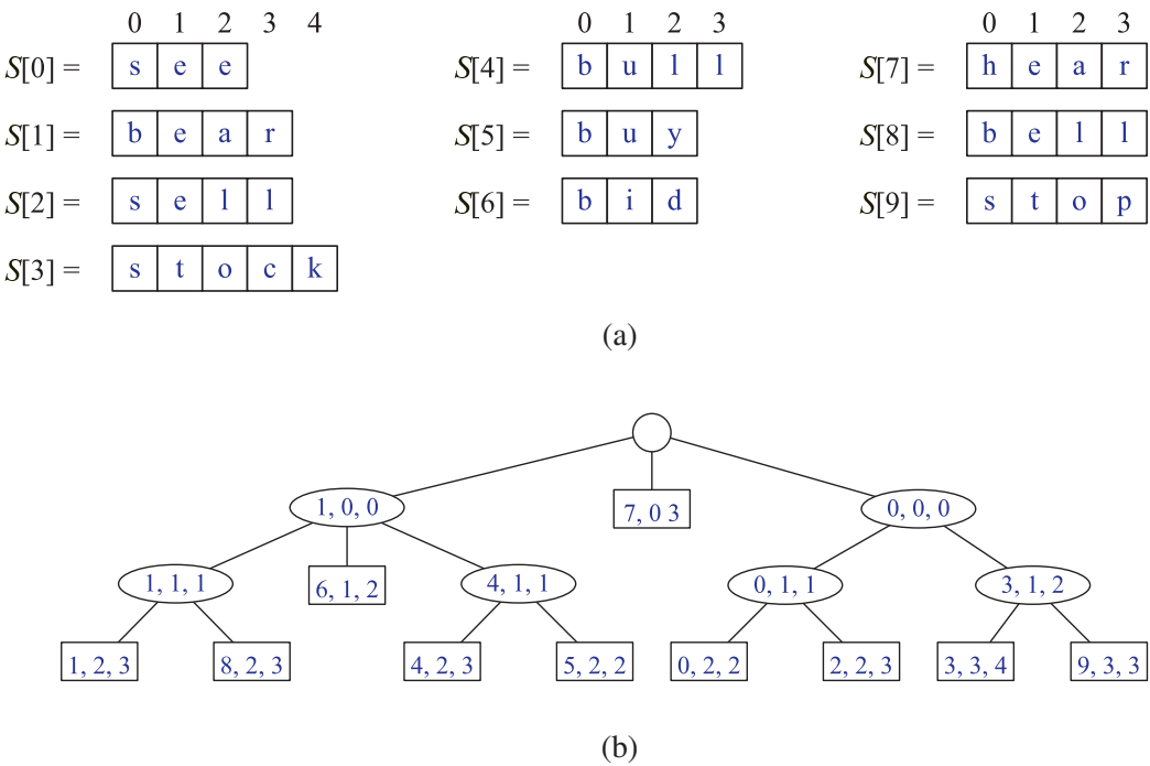
Figure 12.12: (a) Collection S of strings stored in an array. (b) Compact representation of the compressed trie for S .
