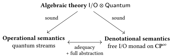
Figure 1. Three semantics of quantum communication and how they relate.
