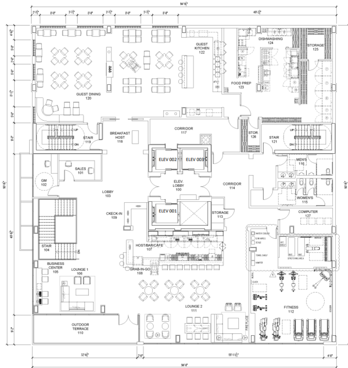
1 LEVEL 1 FLOOR PLAN SCALE: 1/8" = 1'-0"
