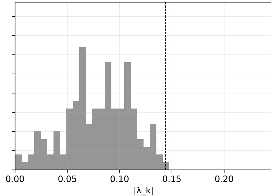
Phase-randomized \rho(A) = 0.144
