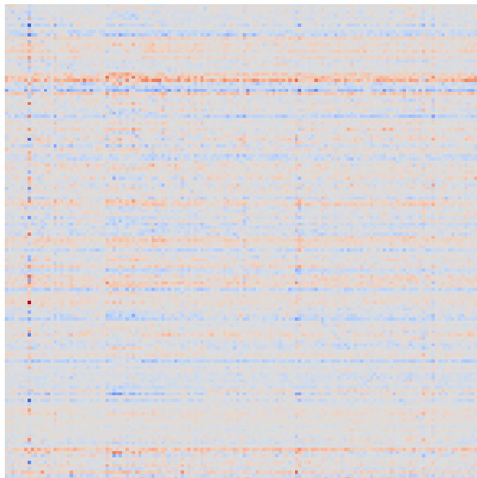
Real data R^2 = 0.038 ( \|A\| = 4.48 )
