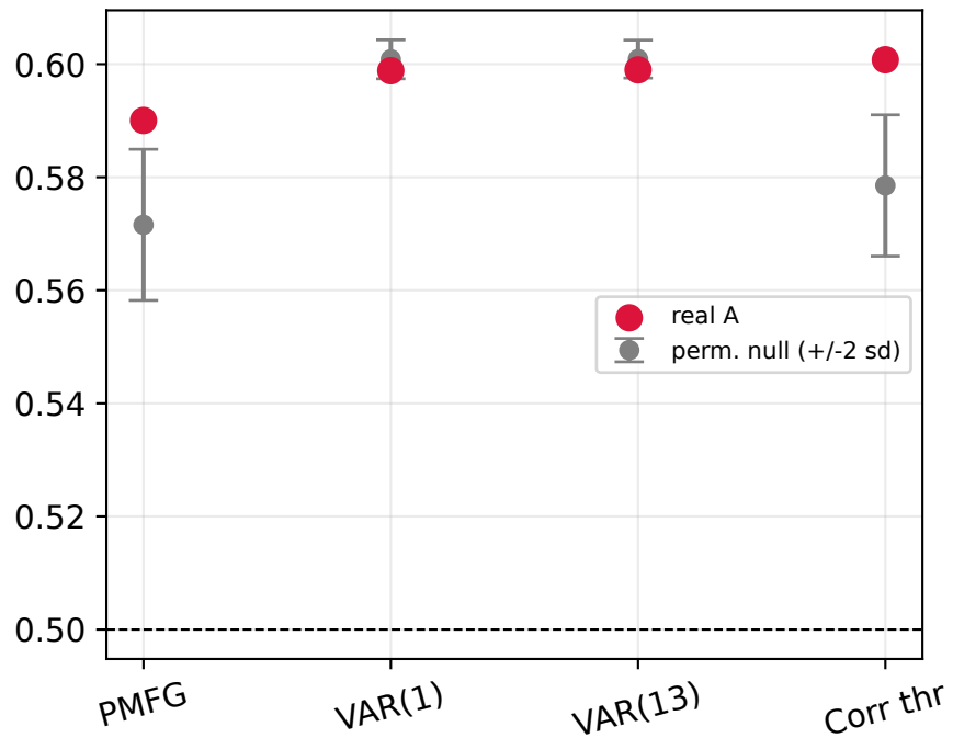
(b) ignition AUC vs permutation null
