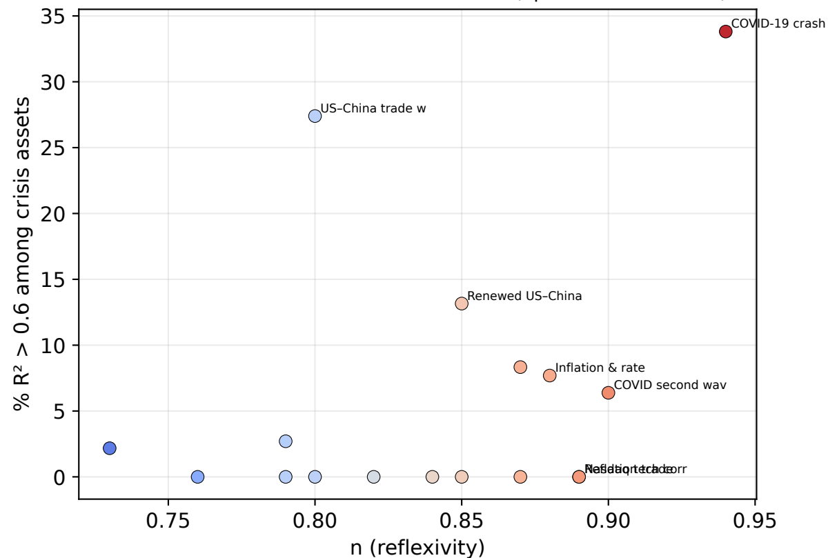
n vs SIS contamination within the crisis set (Spearman rho = 0.25)
