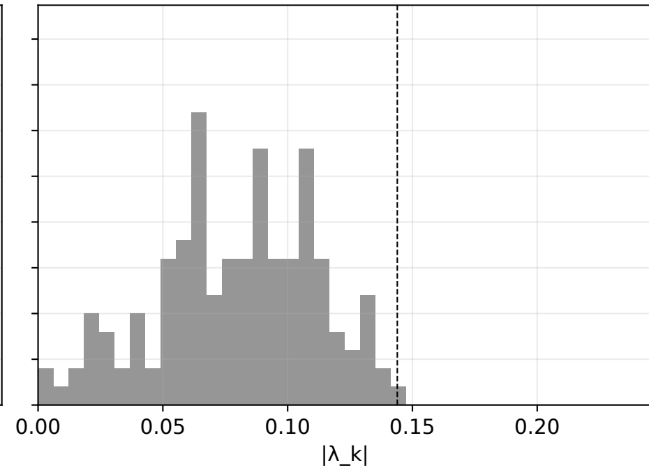
Phase-randomized \rho(A) = 0.144
