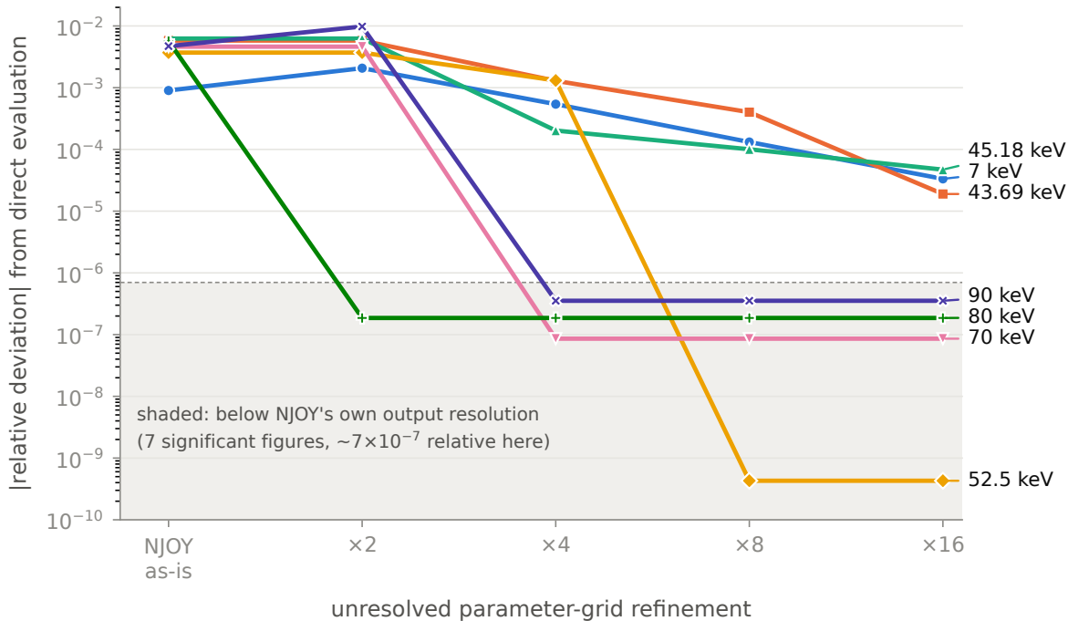
NJOY2016's unresolved-range output converges onto direct evaluation U-234 (MAT 9225), MF=3 MT=18, infinitely dilute, 0 K
