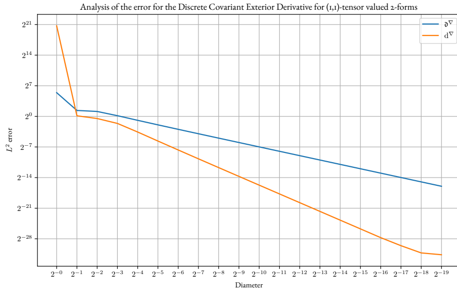
Figure 3.17: Discrete exterior covariant derivative for (1, 1) -tensor-valued 2-forms . As in the (1, 0) - tensor-valued case, we observe that the exterior covariant derivative for (1, 1) -tensor-valued 2-forms converges faster under refinement compared to the PPF-induced discrete exterior covariant derivative.
