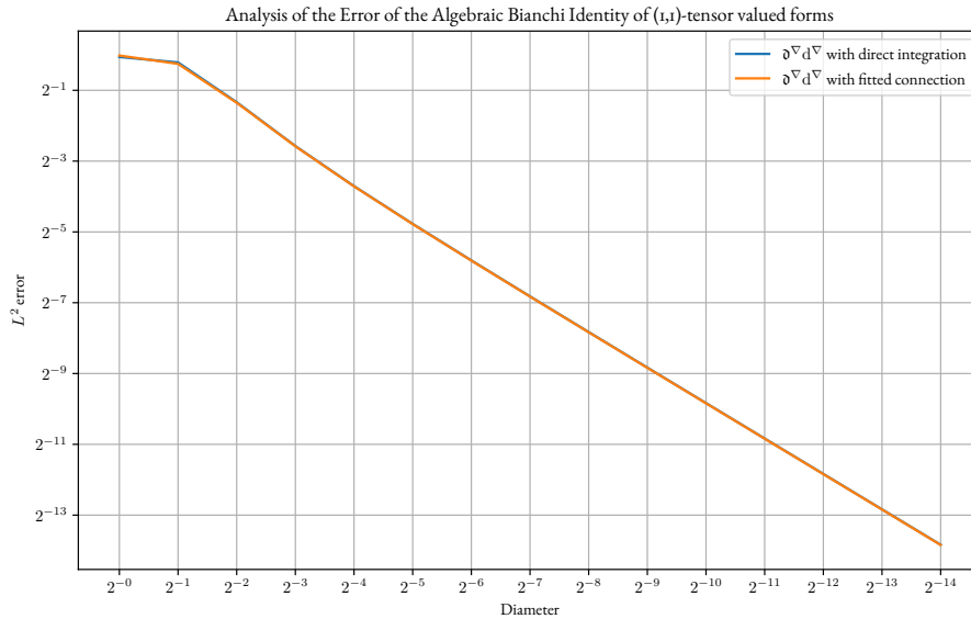
Figure 4.9: Decay of the relative error for the algebraic Bianchi Identity of (1,1) -tensor valued 1-forms In the described setup, we observe that the relative error of the operator d^\nabla d^\nabla converges linearly towards the smooth ground truth.
