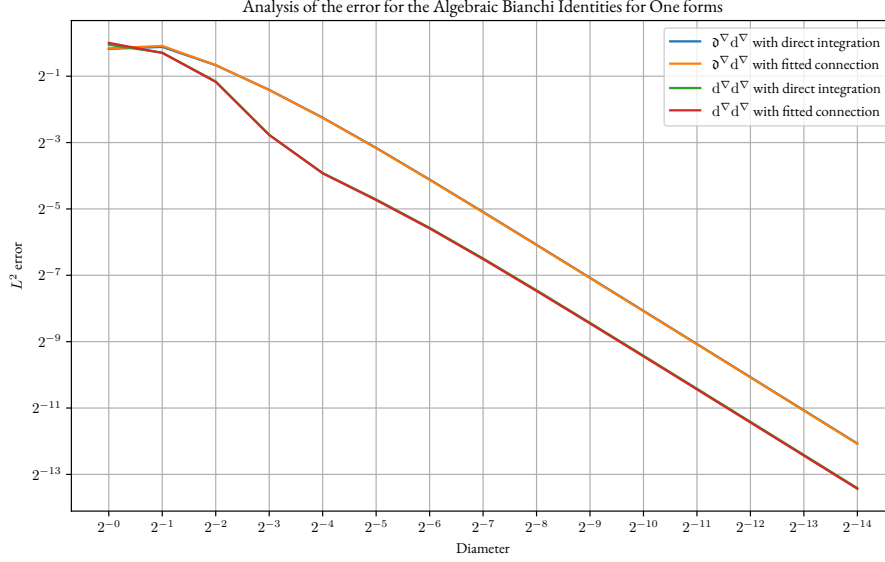
Figure 4.5: Decay of the error for the algebraic Bianchi identity of bundle-valued one-forms We observe that if we use a direct integral of a known smooth connection or fit linearly a connection 1-form on the data available on primal edges to calculate parallel transport to calculate two consecutive applications of the discrete exterior covariant derivative. As in the simplicial case, the operator d^\nabla d^\nabla has the same convergence order as the operator \mathfrak{d}^\nabla d^\nabla under mesh refinement.
