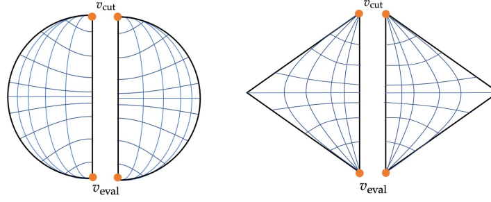
Figure 3.8: Summing Curvatures. For two triangles using the same two prongs (v_{\text{cut}}, v_{\text{eval}}) , the curvature evaluated over their union will be the sum of the curvatures with the same two prongs because the parallel-propagated frames derived from these two prongs properly align.
