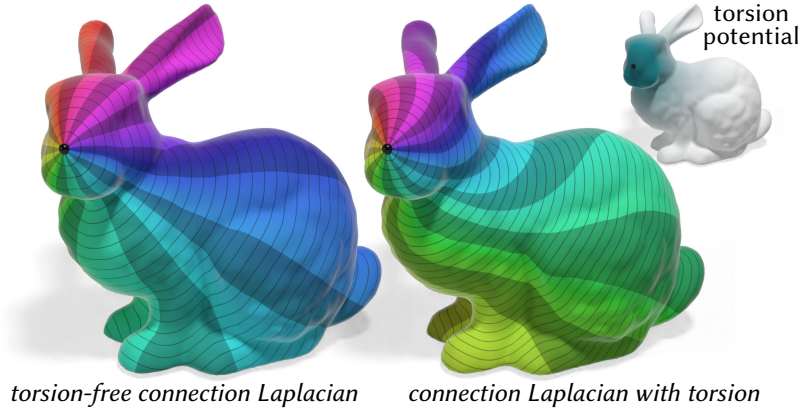
Figure 2.5: Torsion-controlled vector heat method. The connection Laplacian used in the vector heat method of [?] can be formed for any connection. In this example, we compute a logarithmic map—a sort of global polar parameterization—using the connection Laplacian of an ordinary torsion-free connection ( left ), and using a connection with prescribed non-zero torsion equal to the gradient of a torsion potential ( right ), which introduces a distinct twist into the radial lines of the parameterization.
