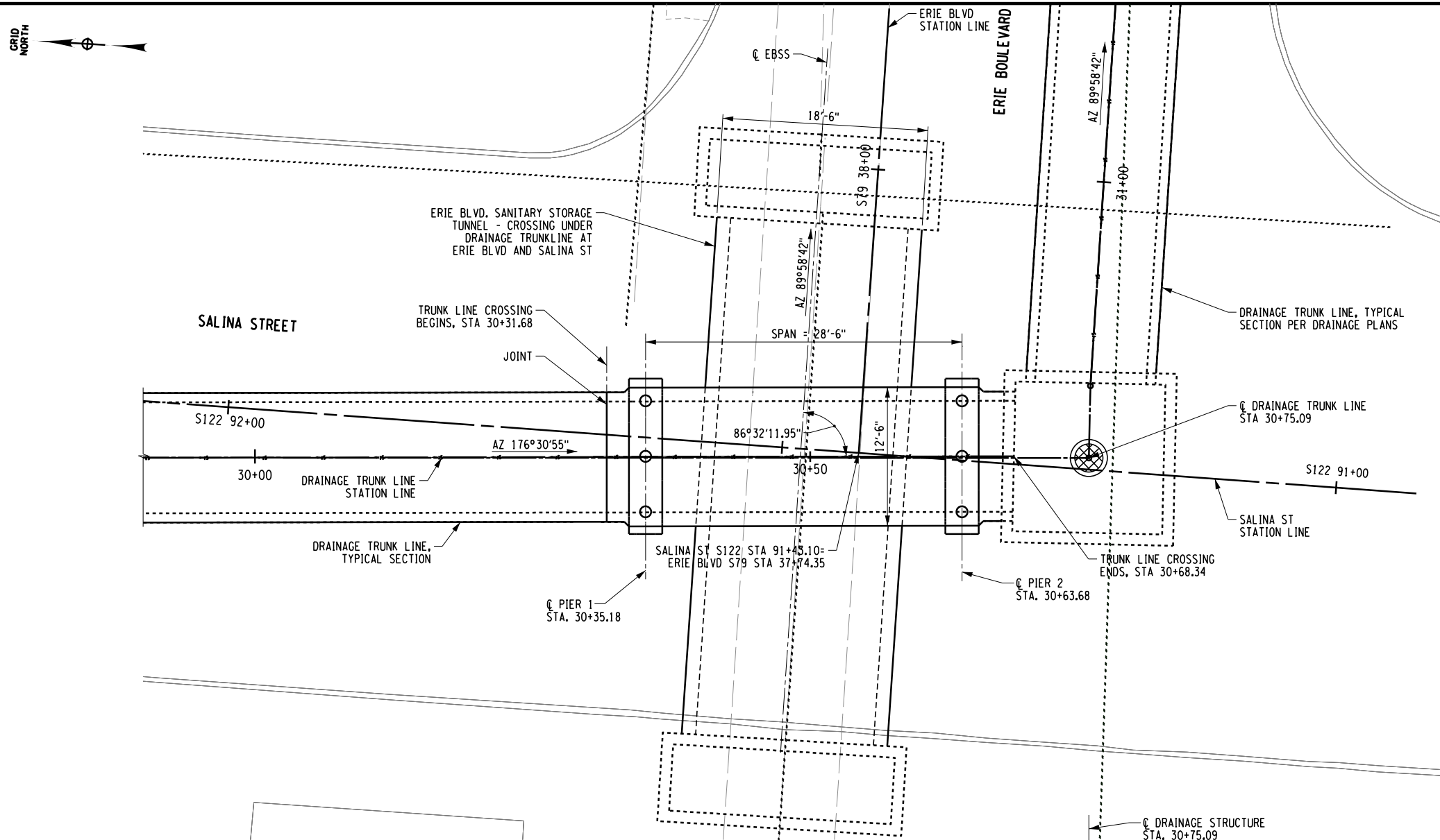
EBSS CROSSING 1 - PLAN VIEW
