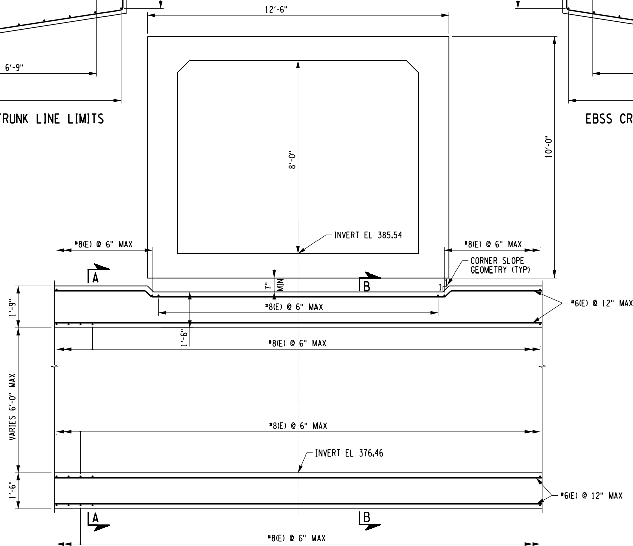
EBSS CROSSING 1 - LONGITUDINAL EBSS SECTION
