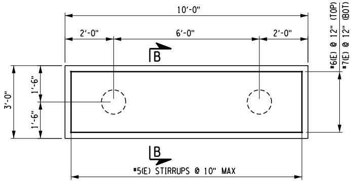
DRAINAGE TRUNK LINE EBSS CROSSING 2 - PILE CAP PLAN
