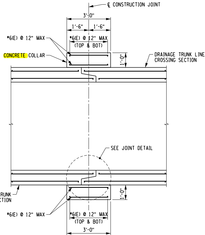
DRAINAGE TRUNK LINE COLLAR - SECTION NTS
