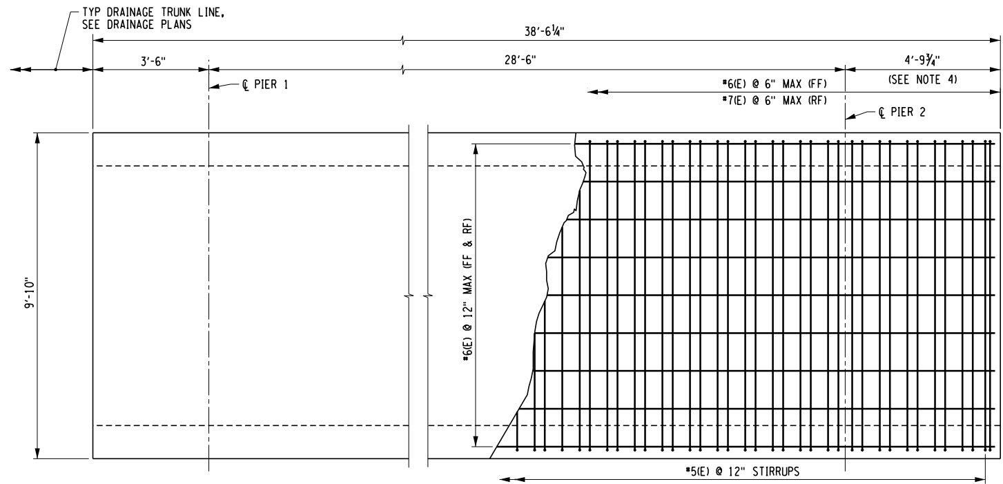
DRAINAGE TRUNK LINE - EBSS CROSSING 1 ELEVATION VIEW
