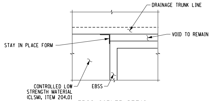
EBSS CORNER DETAIL NTS
