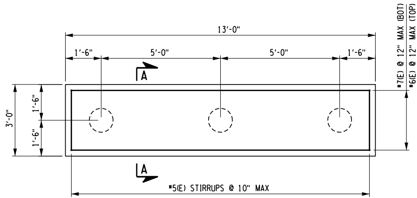
DRAINAGE TRUNK LINE EBSS CROSSING 1 - PILE CAP PLAN
