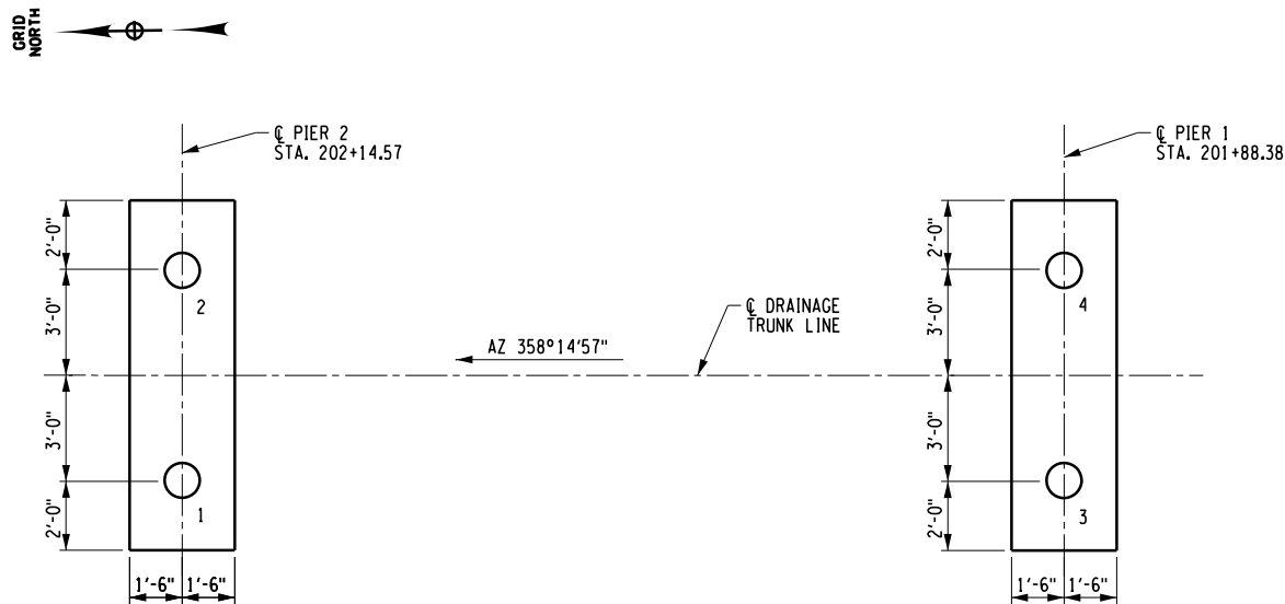
DRAINAGE TRUNK LINE EBSS CROSSING 2 - PILE LAYOUT PLAN
