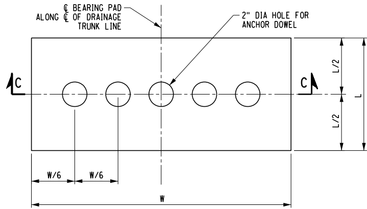
PLAN PLAIN ELASTOMERIC BEARING (TYPE E.P.)
