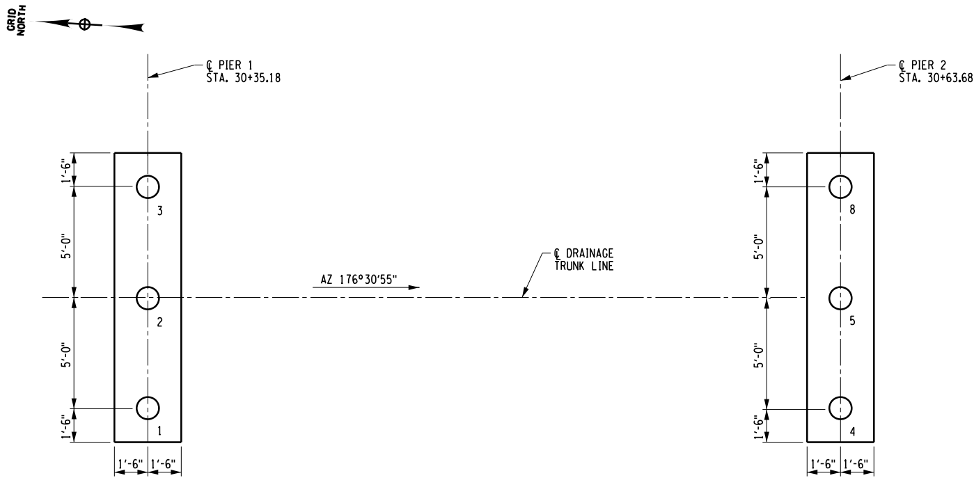
DRAINAGE TRUNK LINE EBSS CROSSING 1 - PILE LAYOUT PLAN
