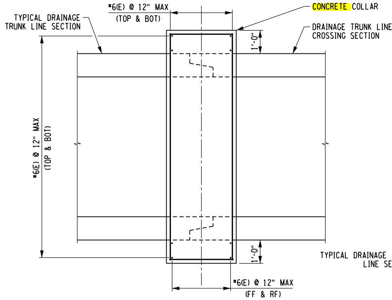
DRAINAGE TRUNK LINE COLLAR - PLAN NTS
