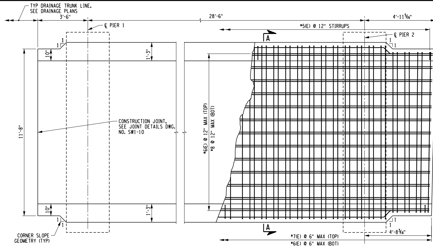
DRAINAGE TRUNK LINE - EBSS CROSSING 1 BOTTOM SLAB PLAN VIEW
