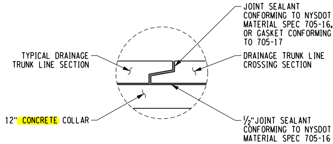
DRAINAGE TRUNK LINE JOINT - DETAIL NTS
