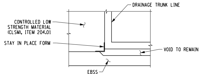
EBSS CORNER DETAIL NTS
