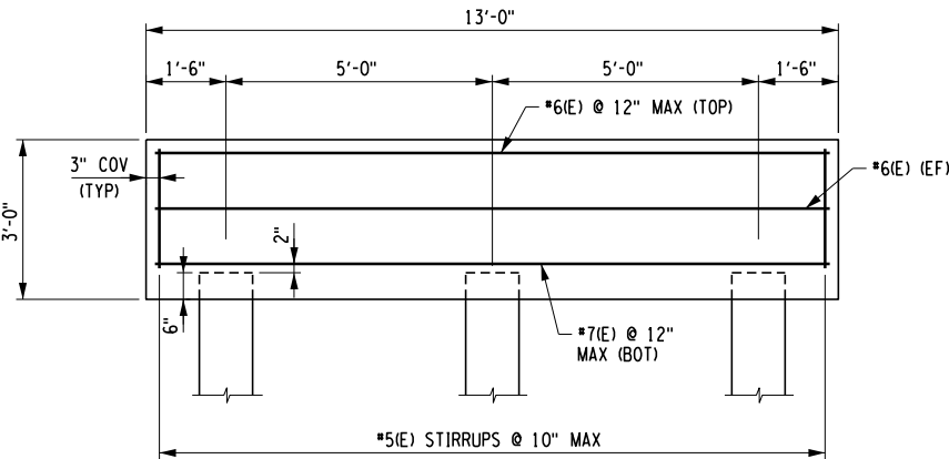
DRAINAGE TRUNK LINE EBSS CROSSING 1 - PILE CAP ELEVATION
