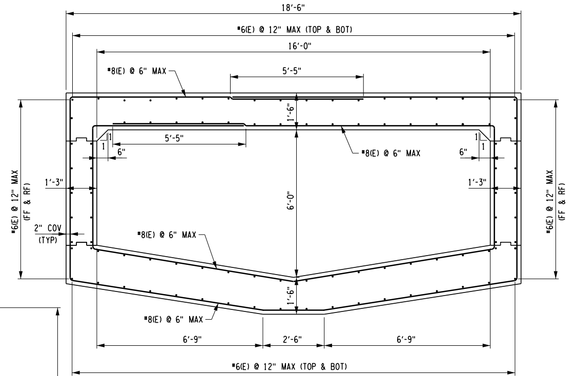
EBSS CROSSING 1 SECTION B - INSIDE DRAINAGE TRUNK LINE LIMITS
