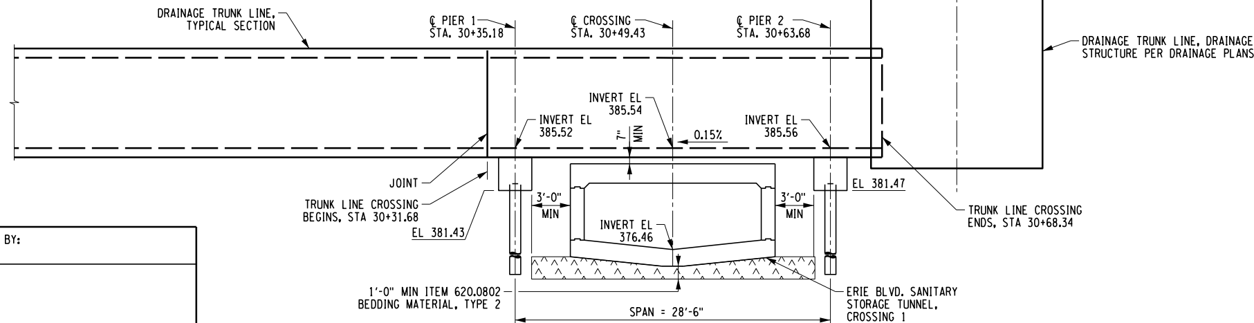
EBSS CROSSING 1 - ELEVATION VIEW
