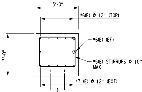
DRAINAGE TRUNK LINE EBSS CROSSING 2 - PILE CAP SECTION B-B
