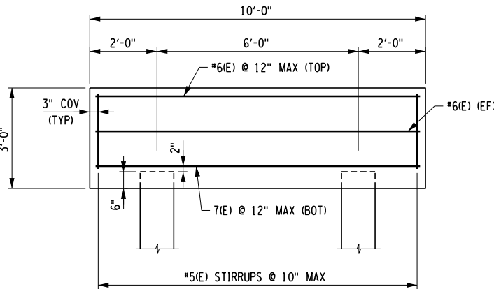
DRAINAGE TRUNK LINE EBSS CROSSING 2 - PILE CAP ELEVATION
