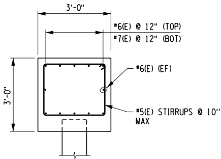
DRAINAGE TRUNK LINE EBSS CROSSING 1 - PILE CAP SECTION A-A
