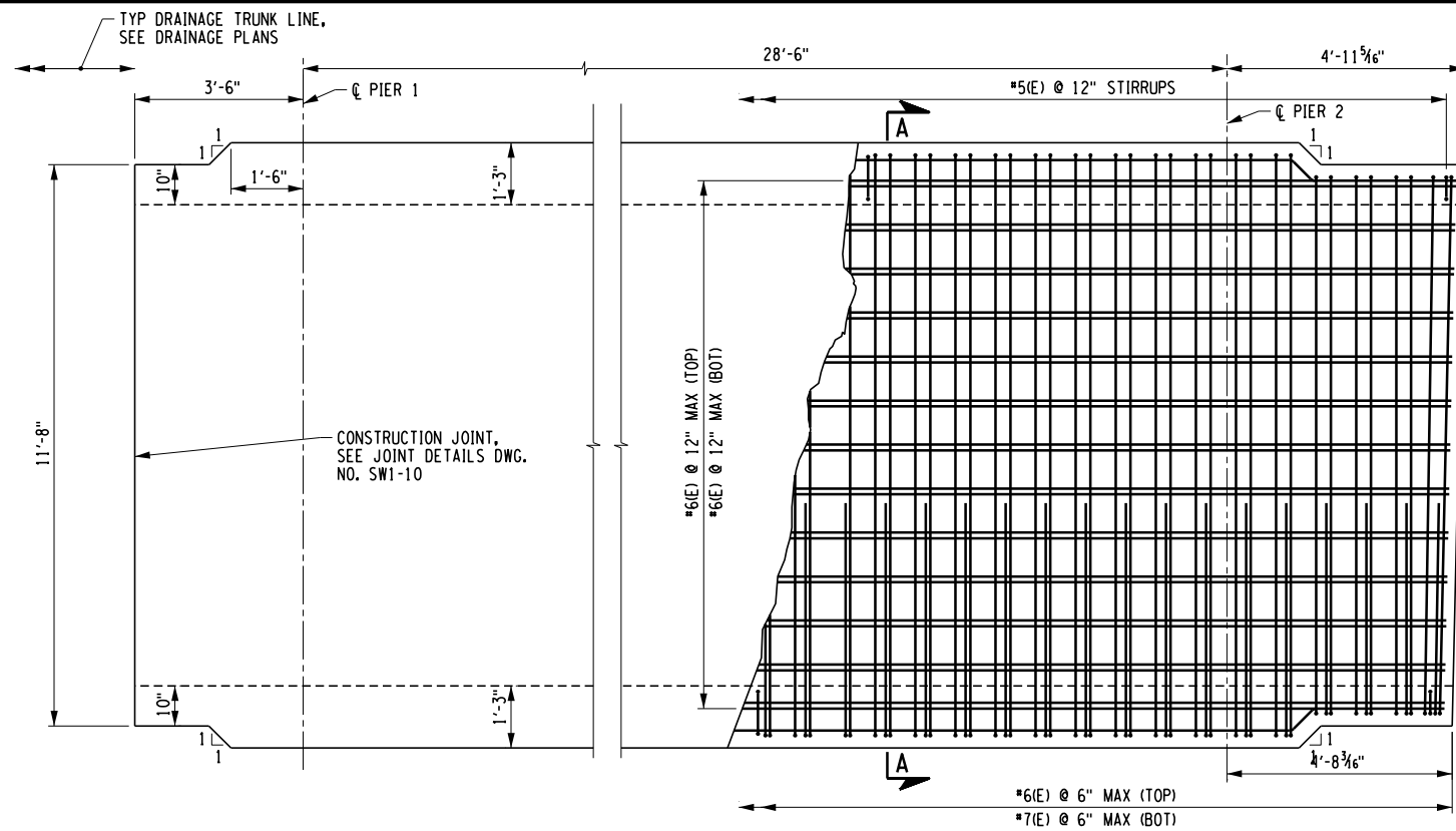
DRAINAGE TRUNK LINE - EBSS CROSSING 1 TOP SLAB PLAN VIEW
