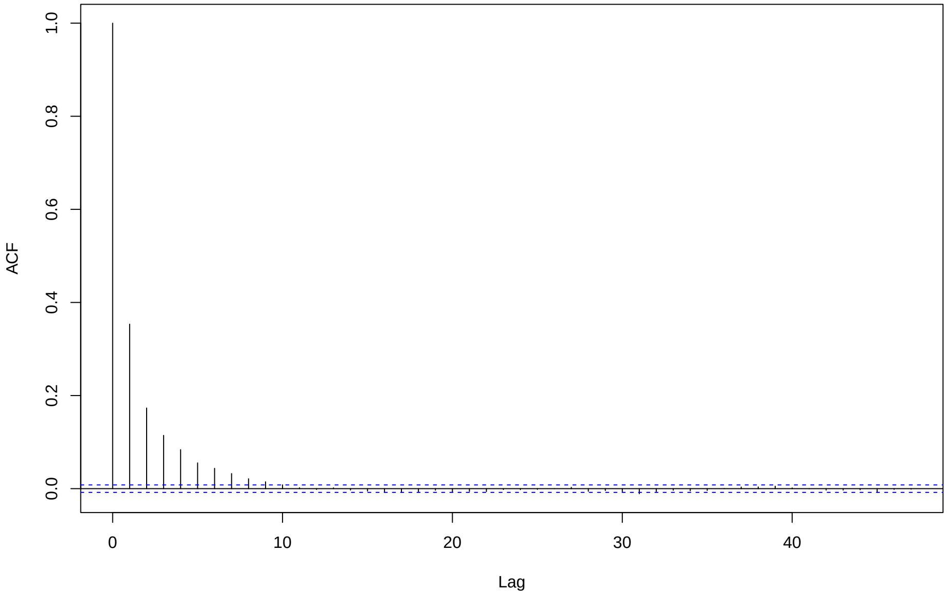
ACF for eta[2,3]
