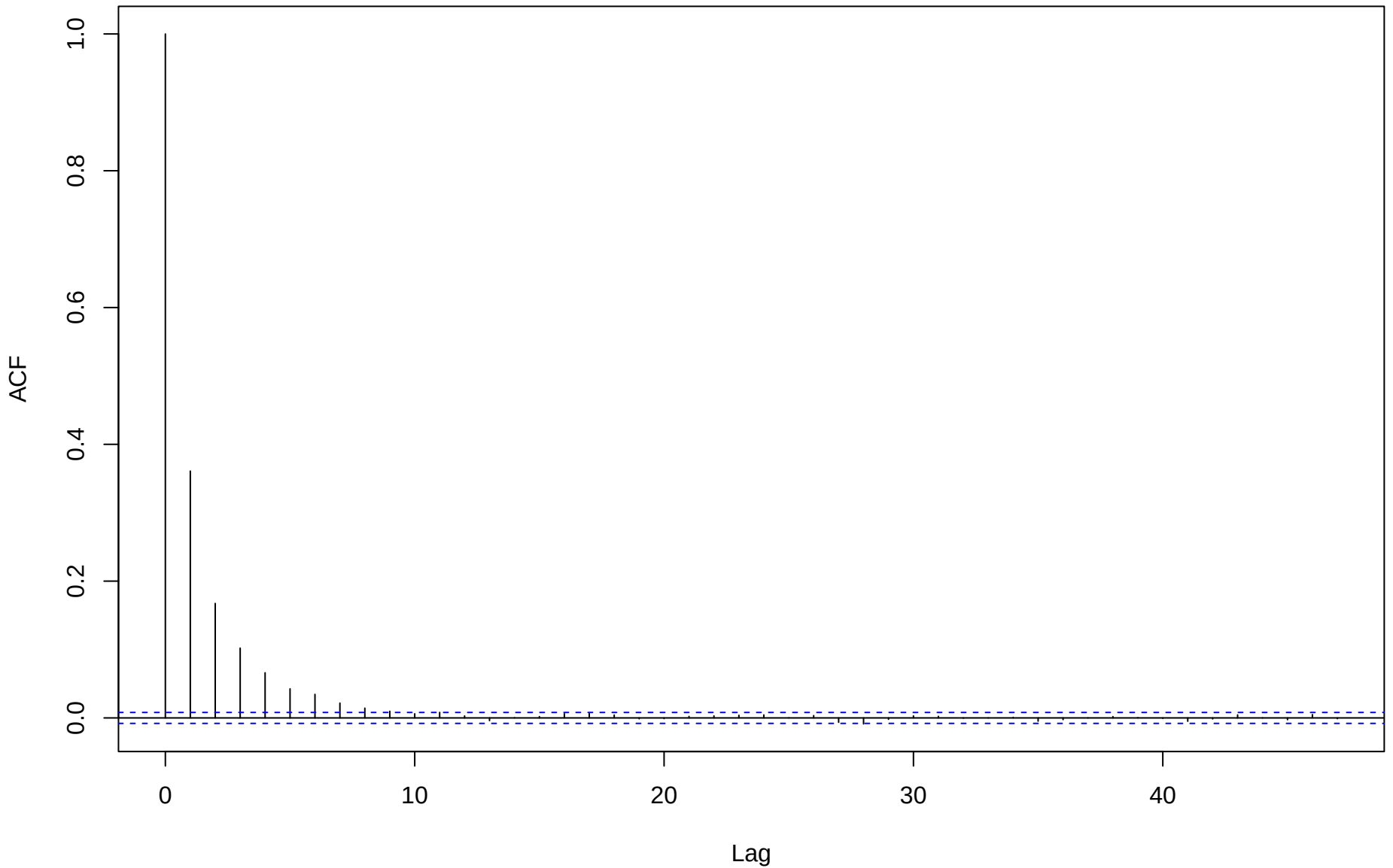
ACF for eta[3,2]
