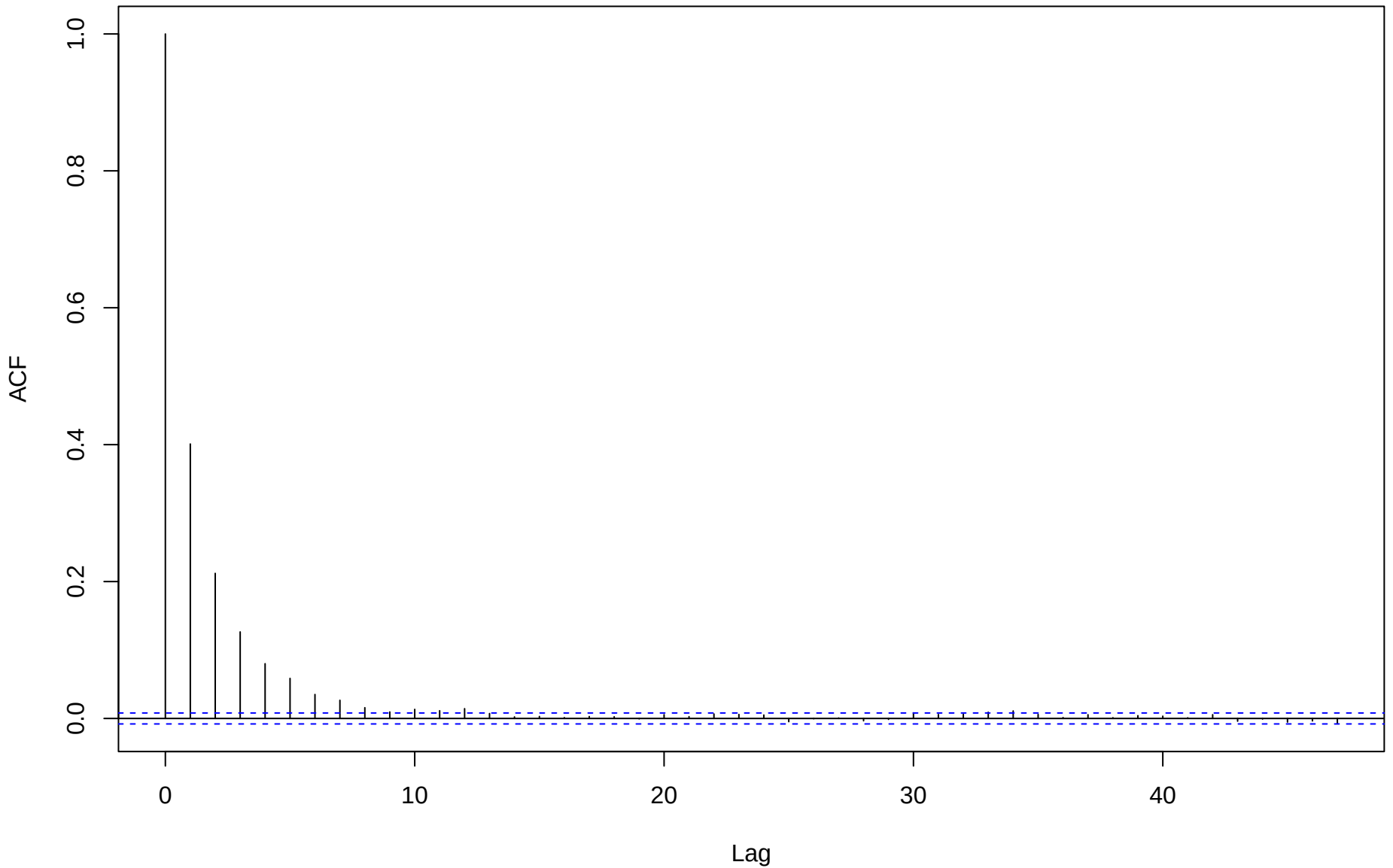
ACF for eta[3,8]
