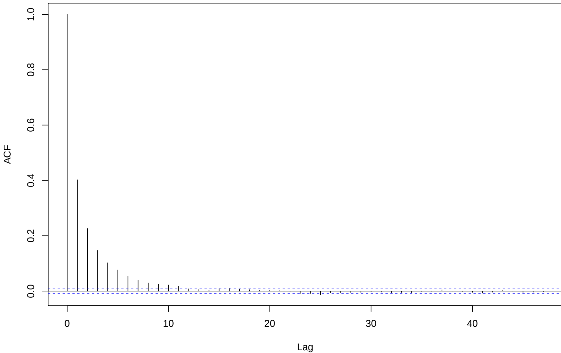
ACF for eta[1,10]
