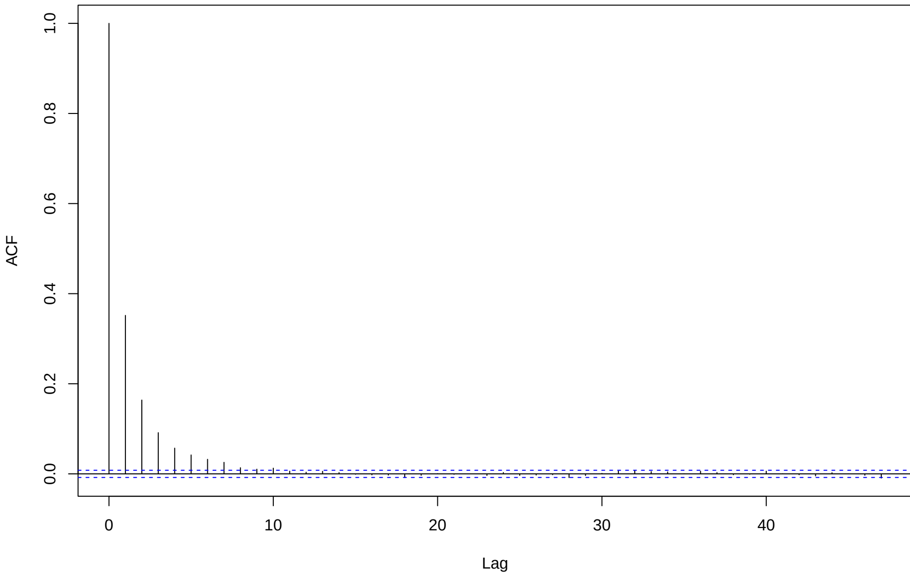
ACF for eta[3,10]
