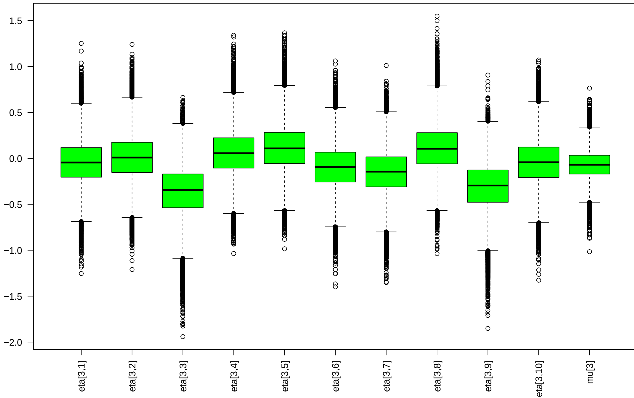
Posterior Boxplots for Sector 3 and \mu
