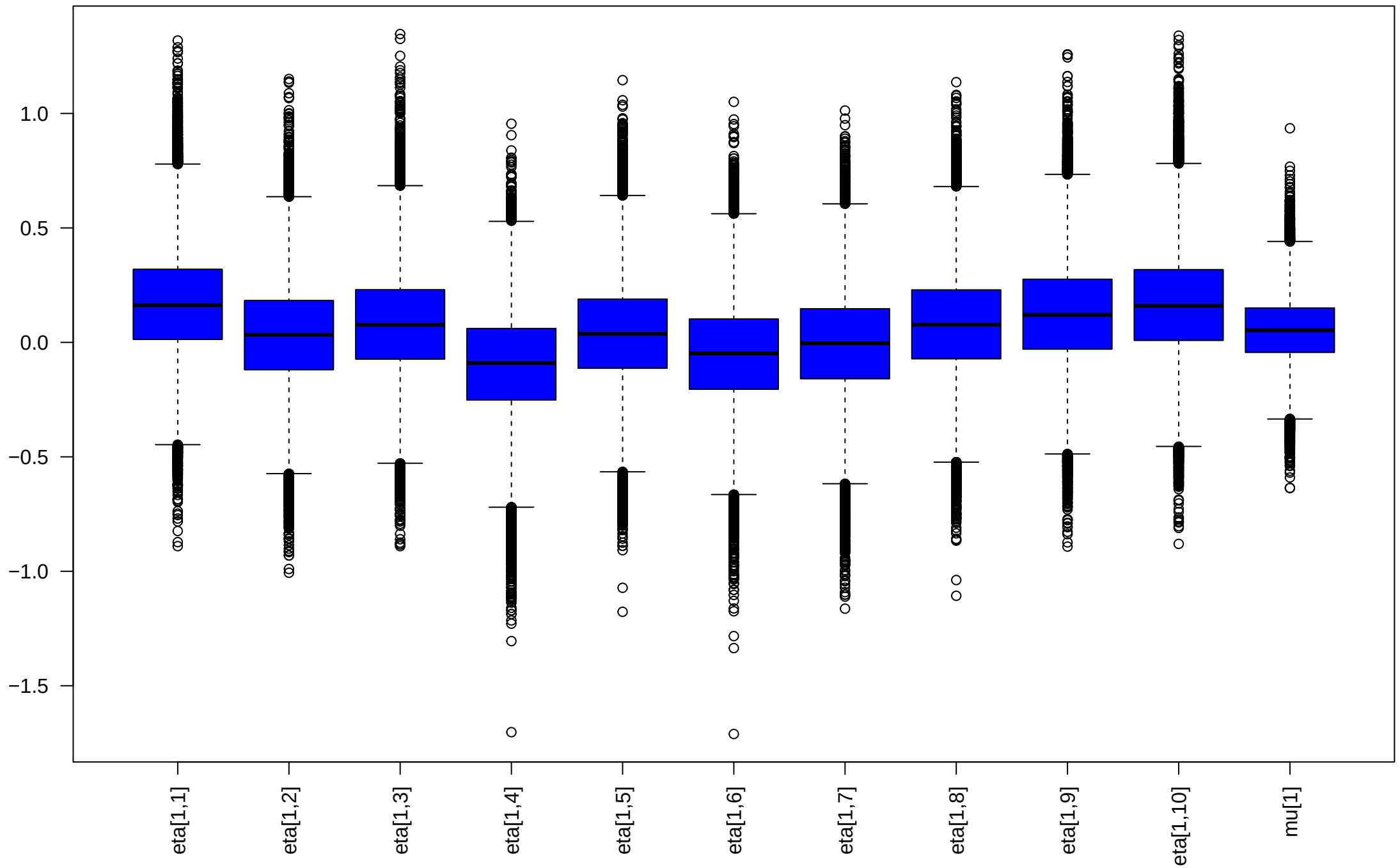
Posterior Boxplots for Sector 1 and \mu
