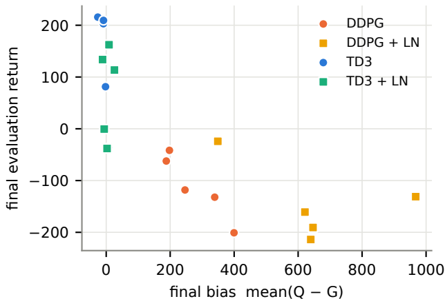
Bias vs. return, one point per run (Spearman \rho = -0.87 , p < 0.001 , n = 20 )
