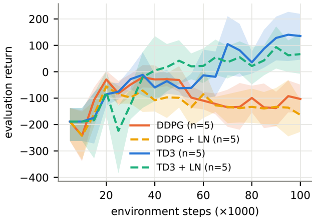
Performance on LunarLanderContinuous
