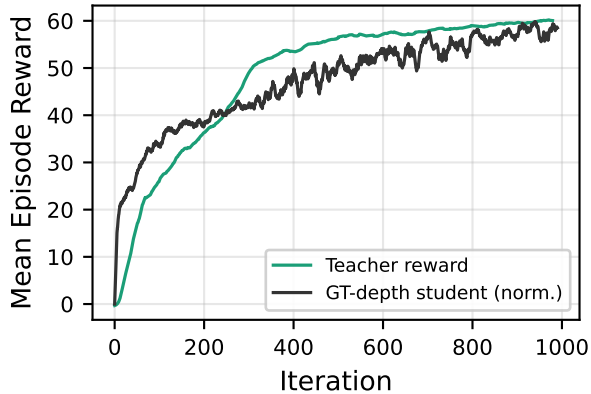
(a) Reward
