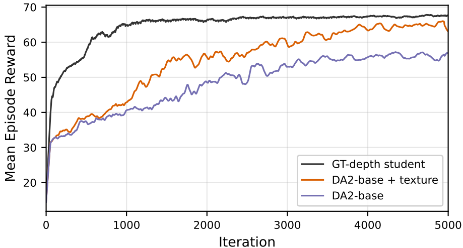
Student Reward During Training
