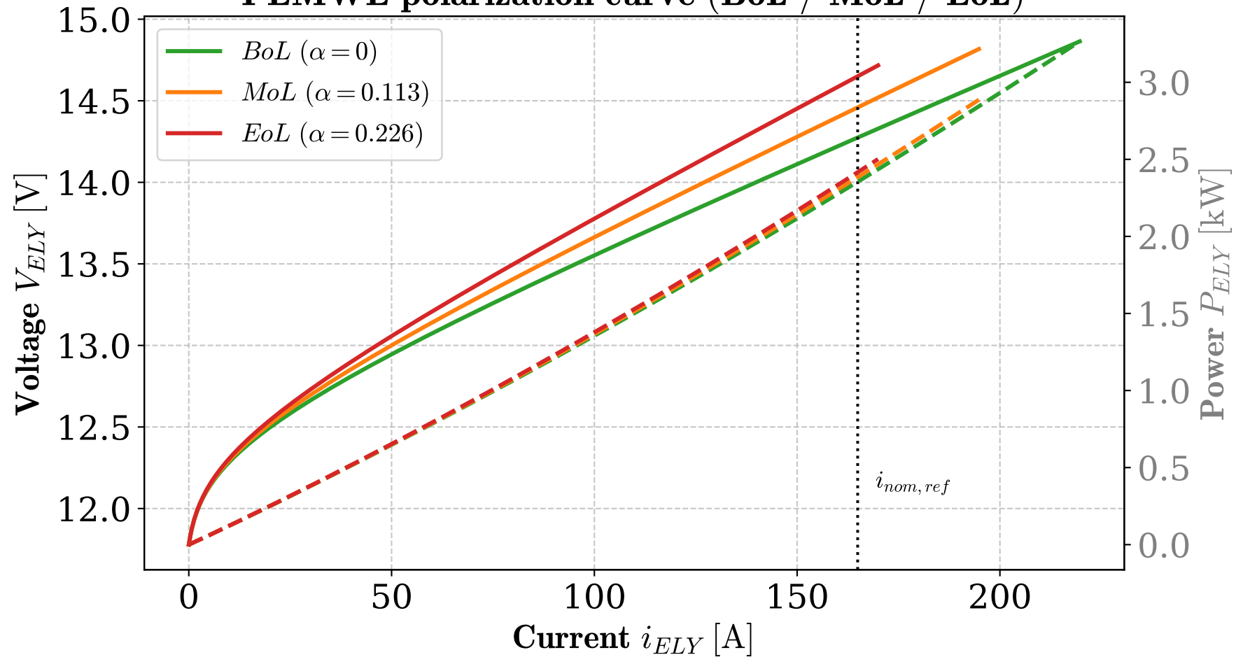
PEMWE polarization curve (BoL / MoL / EoL)
