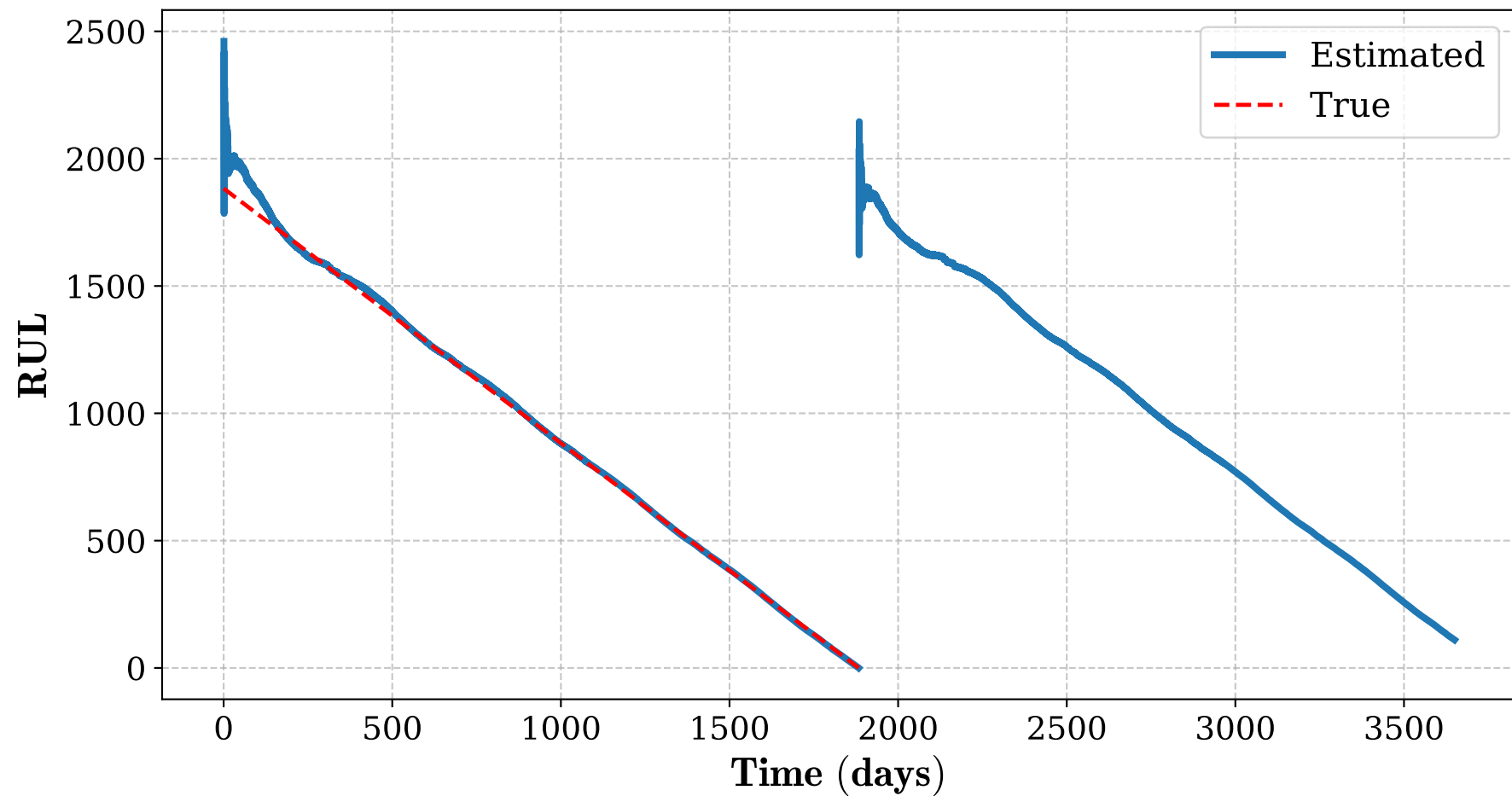
RUL of the fuel cell
