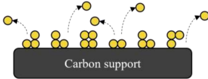
Platinum dissolution
