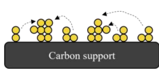
Ostwald ripening
