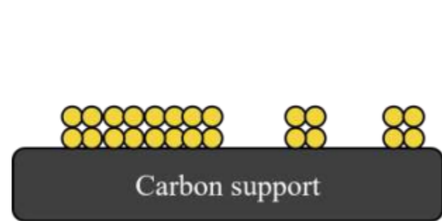
Platinum agglomeration
