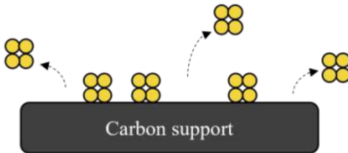
Platinum detachment
