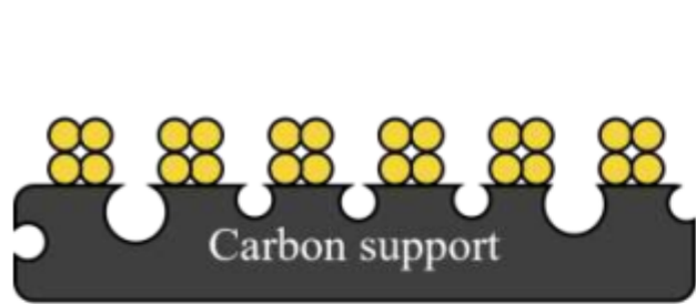
Carbon corrosion
