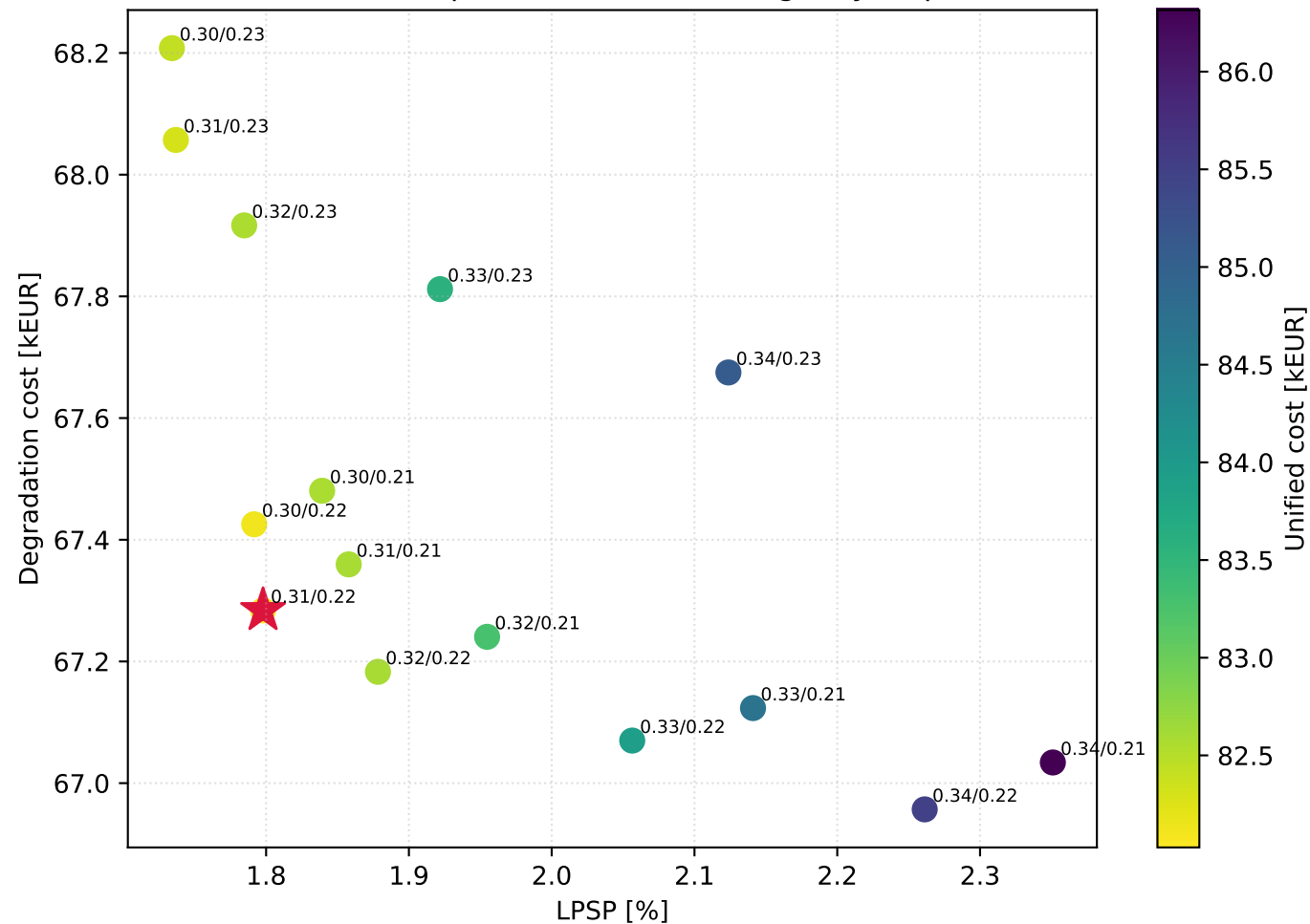
RB2 normal setpoints with SoC emergency dispatch
