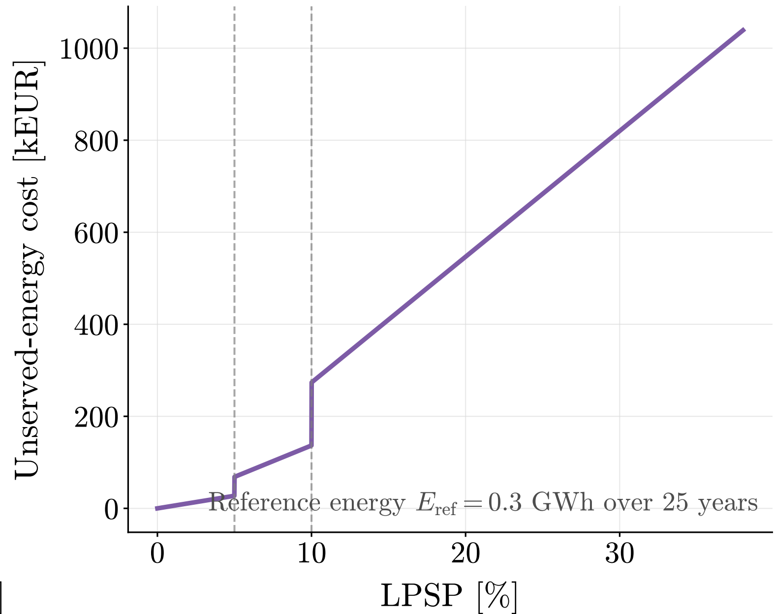
\text{Cost} \propto \text{VOLL}(\text{LPSP}) \times \text{Unserved Energy}
