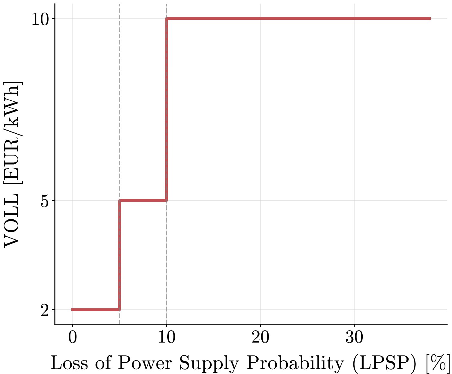
Tiered Value Of Lost Load (VOLL)
