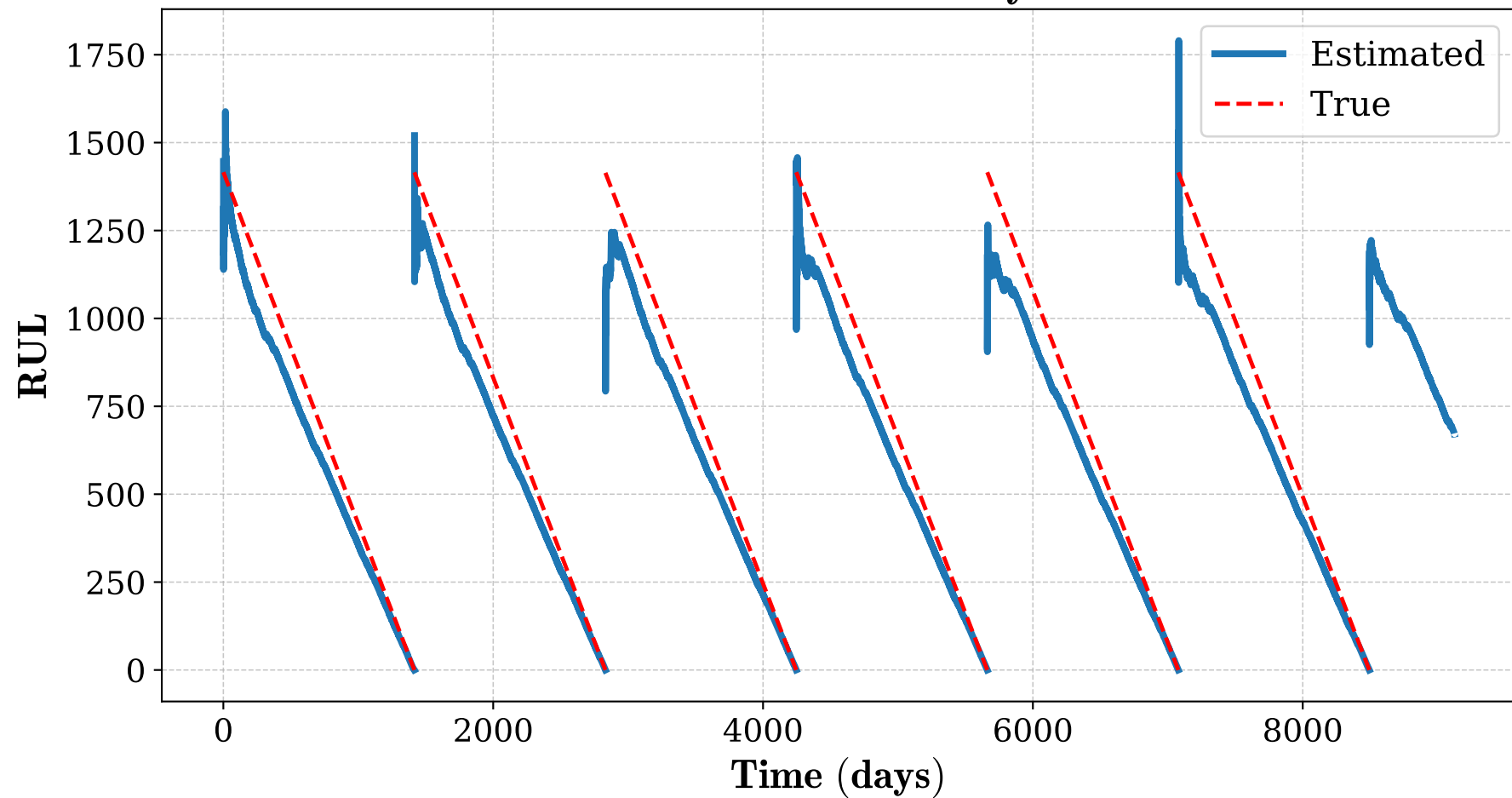
RUL of the battery
