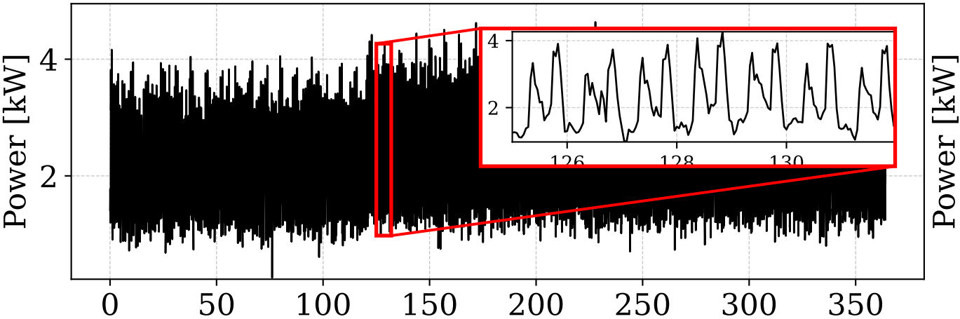
Load profile
