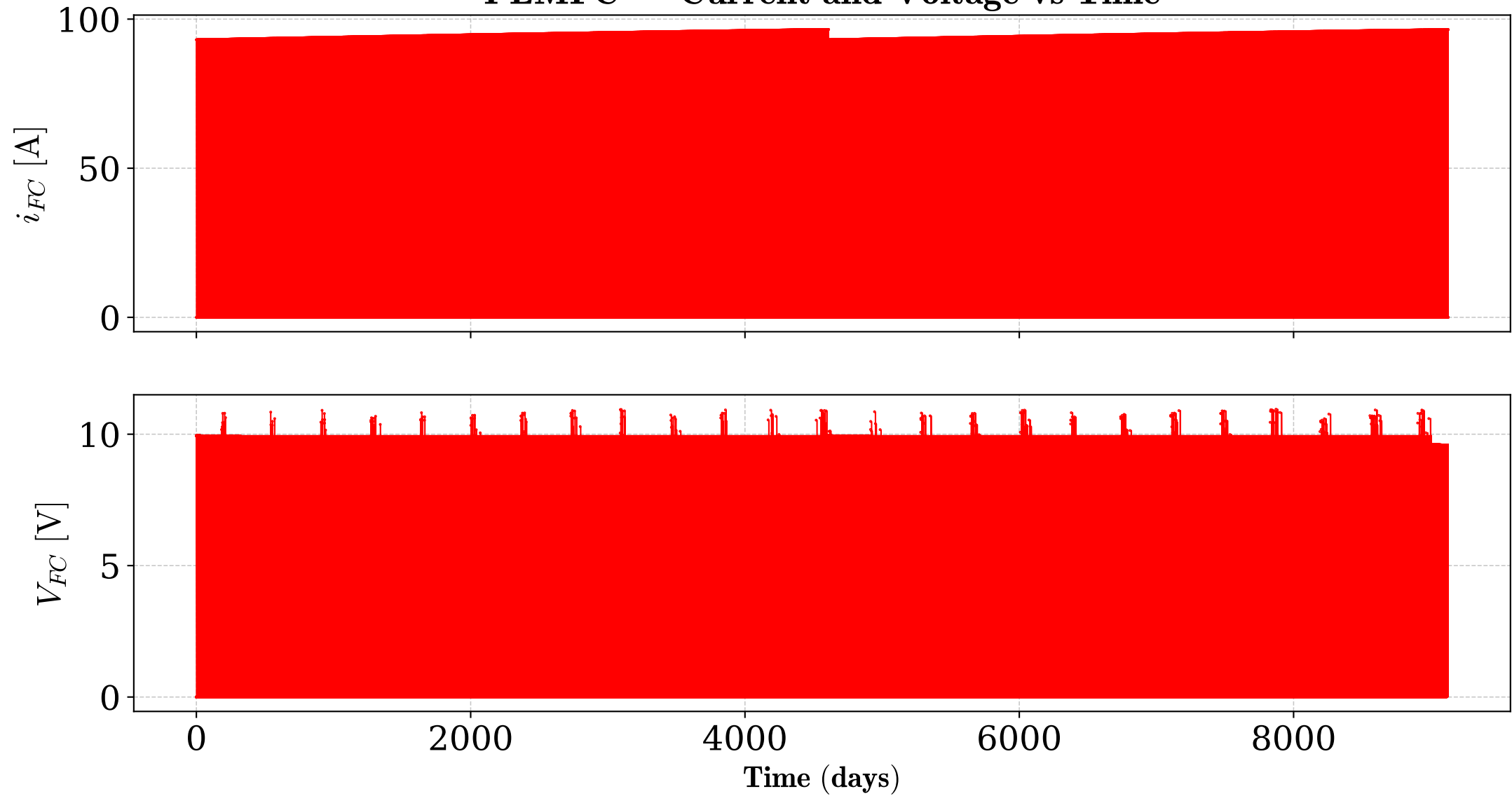
PEMFC — Current and Voltage vs Time
