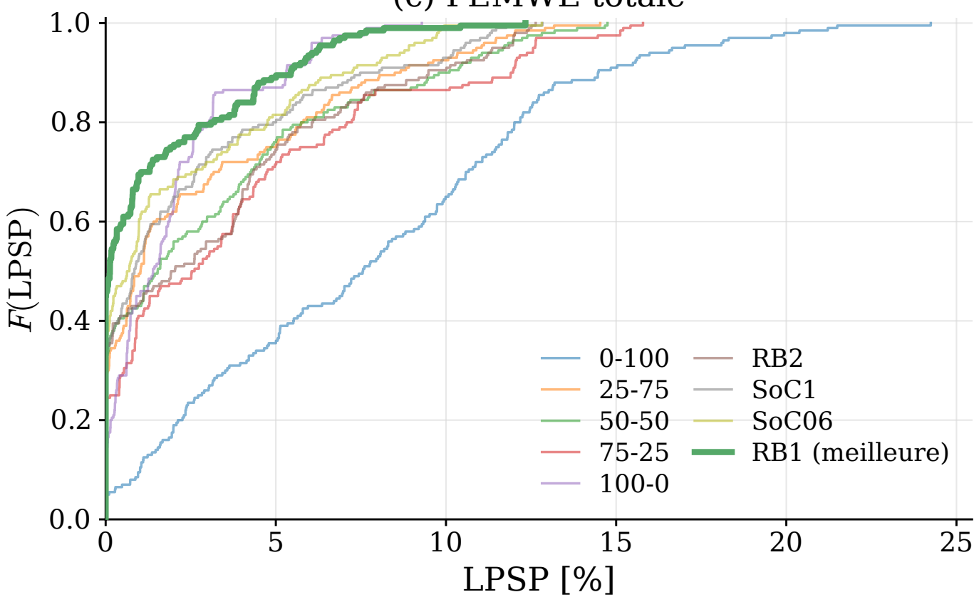
(c) PEMWE totale
