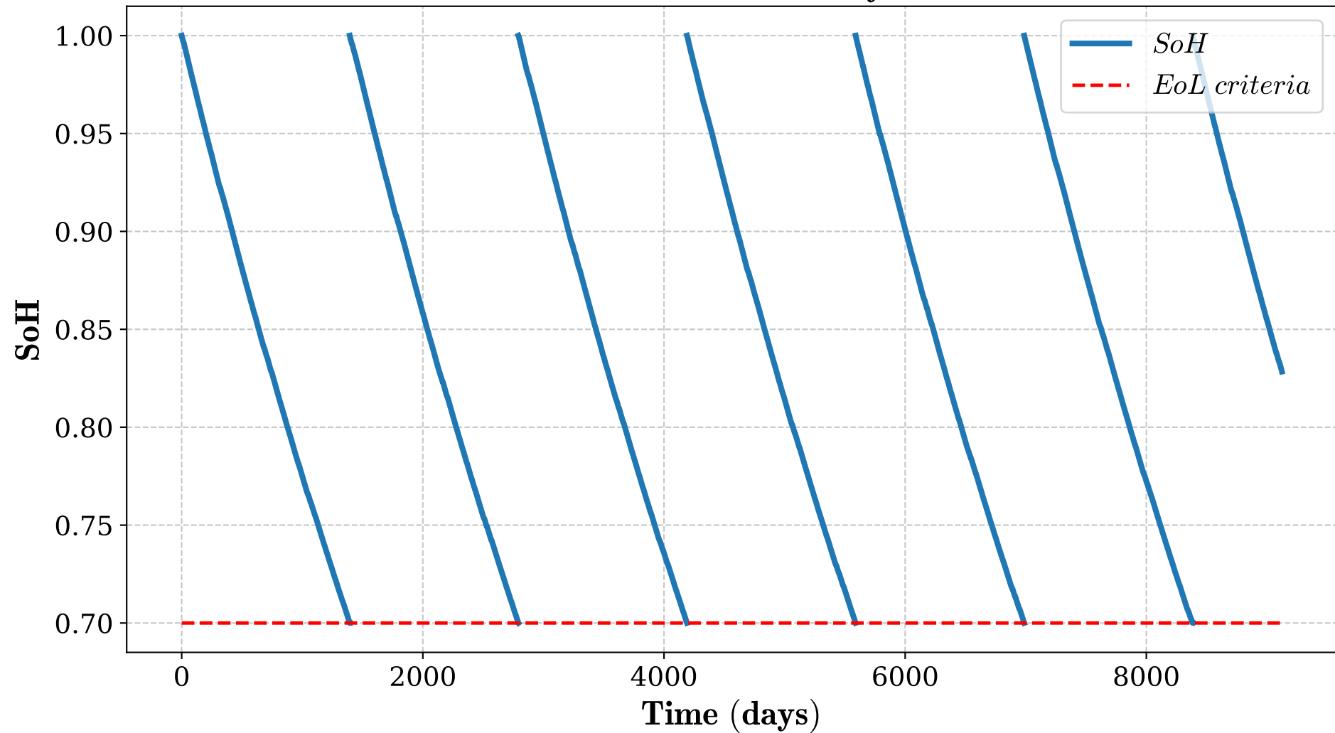
SoH of the battery
