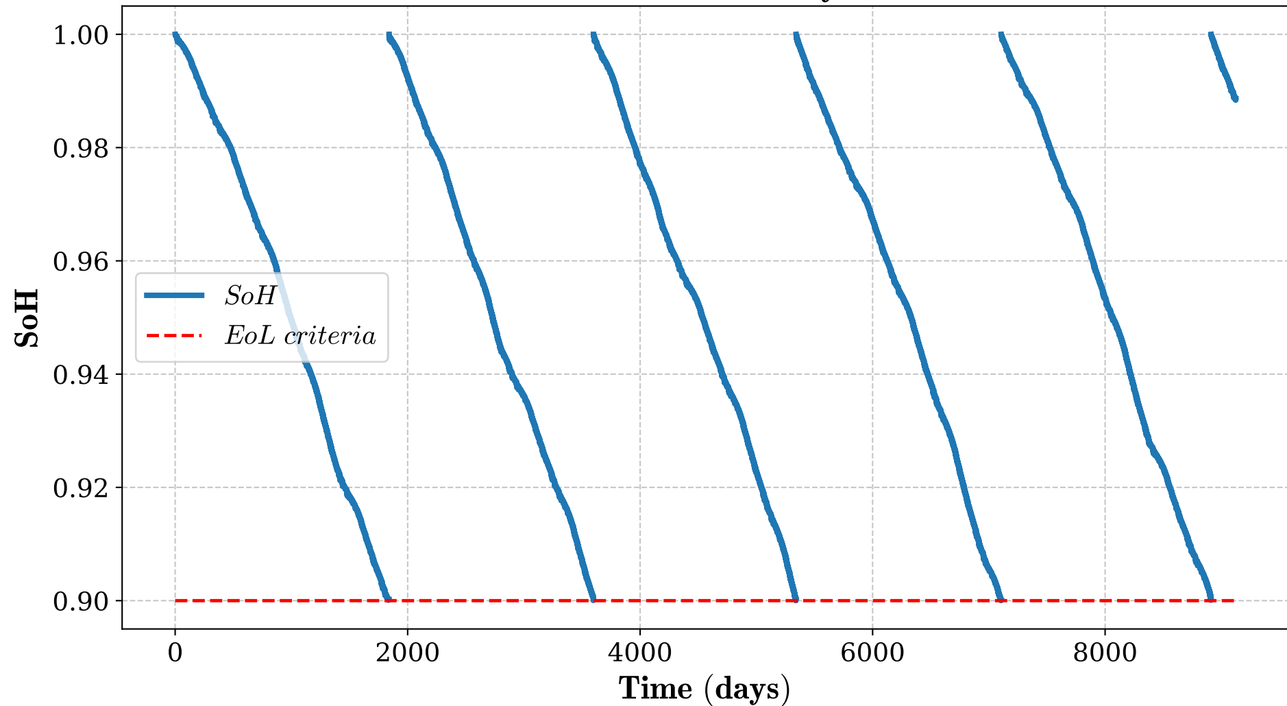
SoH of the electrolyzer
