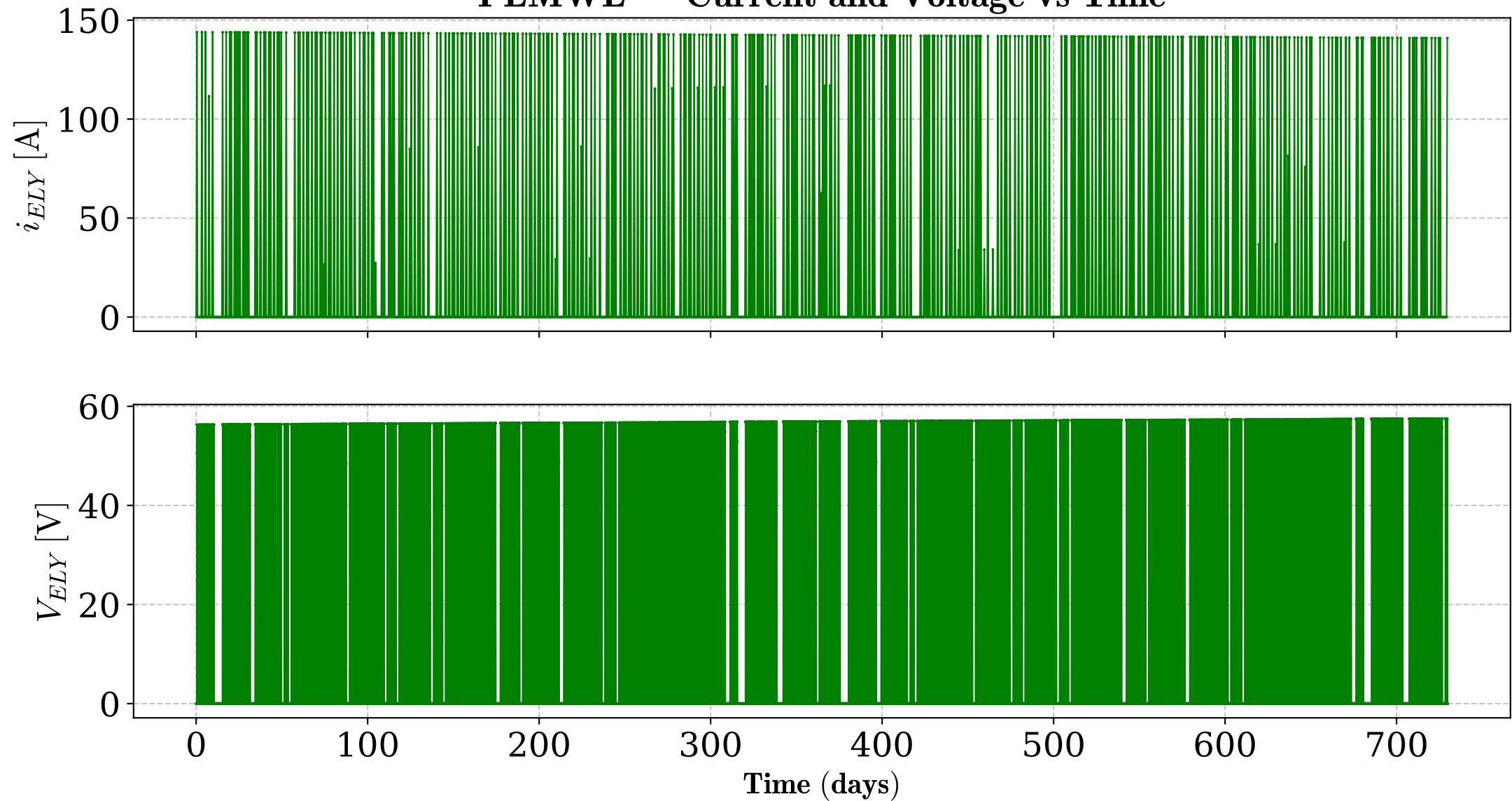
PEMWE — Current and Voltage vs Time
