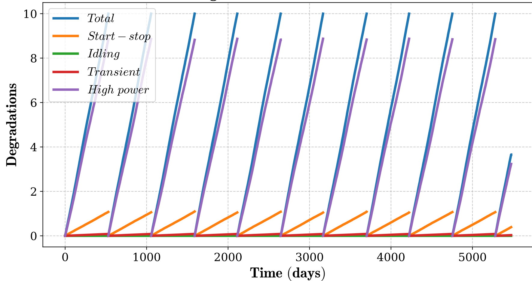
Degradations of the fuel cell
