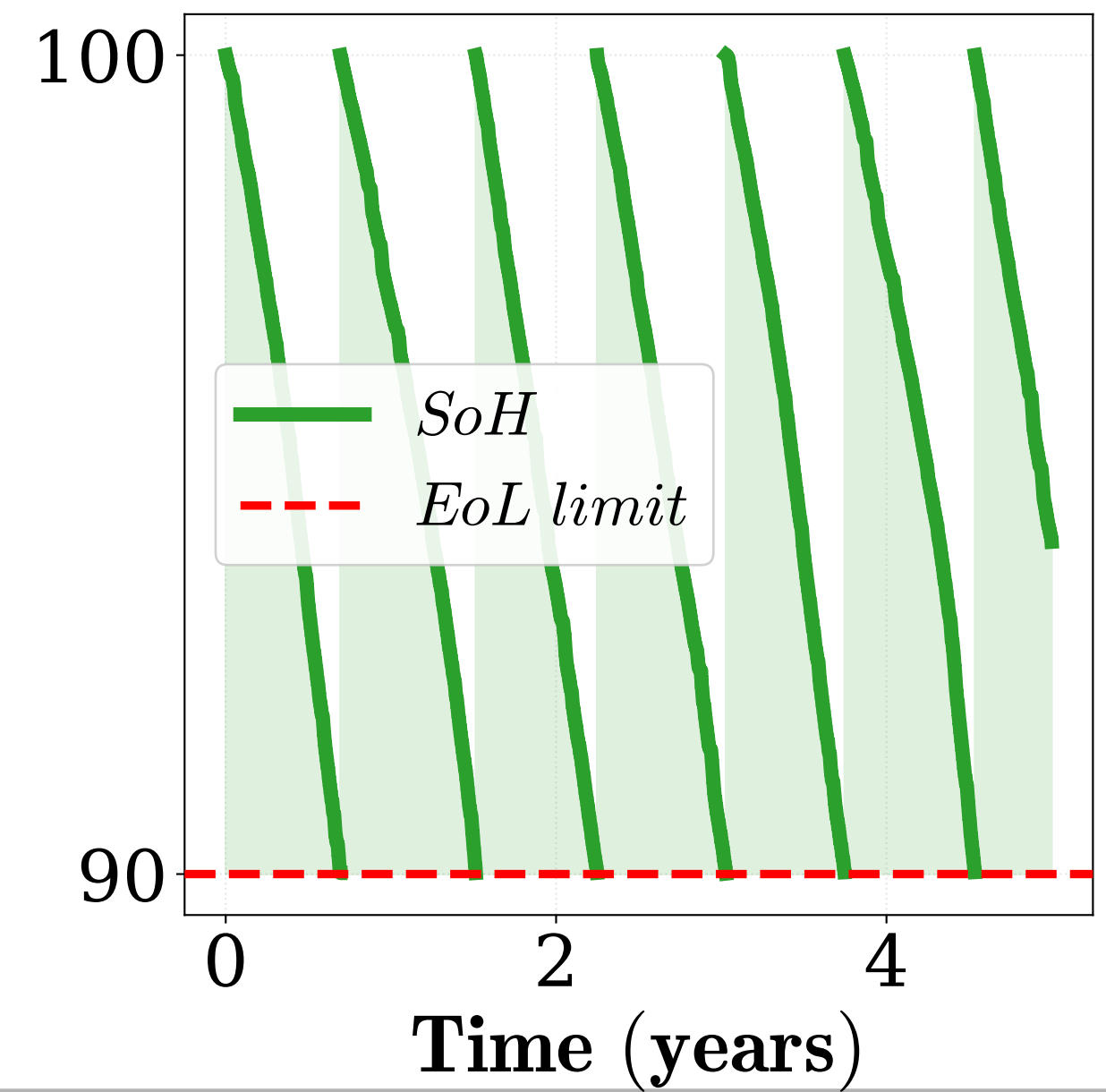
PEMWE Degradation High power
