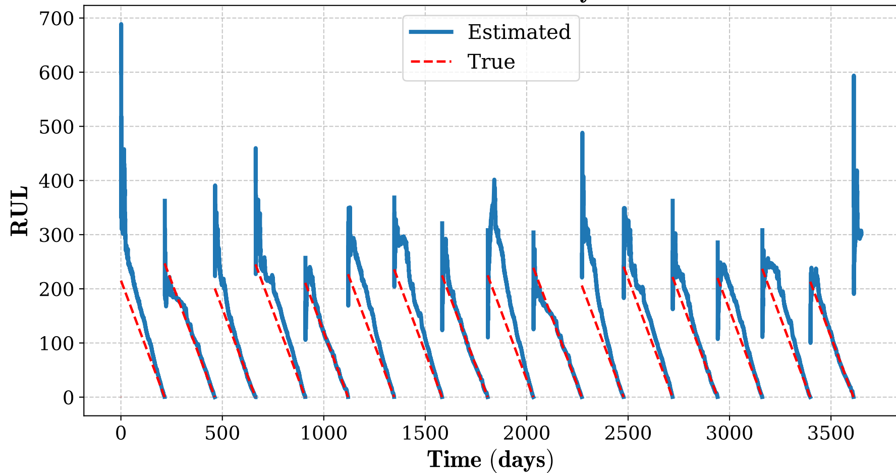
RUL of the electrolyzer
