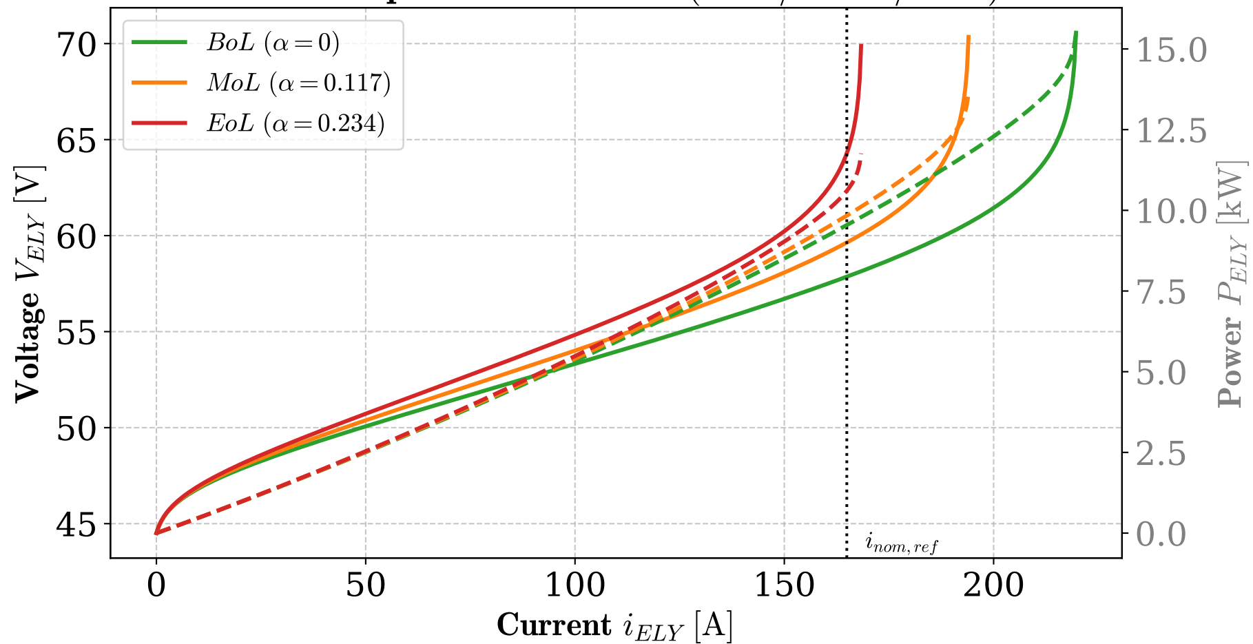
PEMWE polarization curve (BoL / MoL / EoL)
