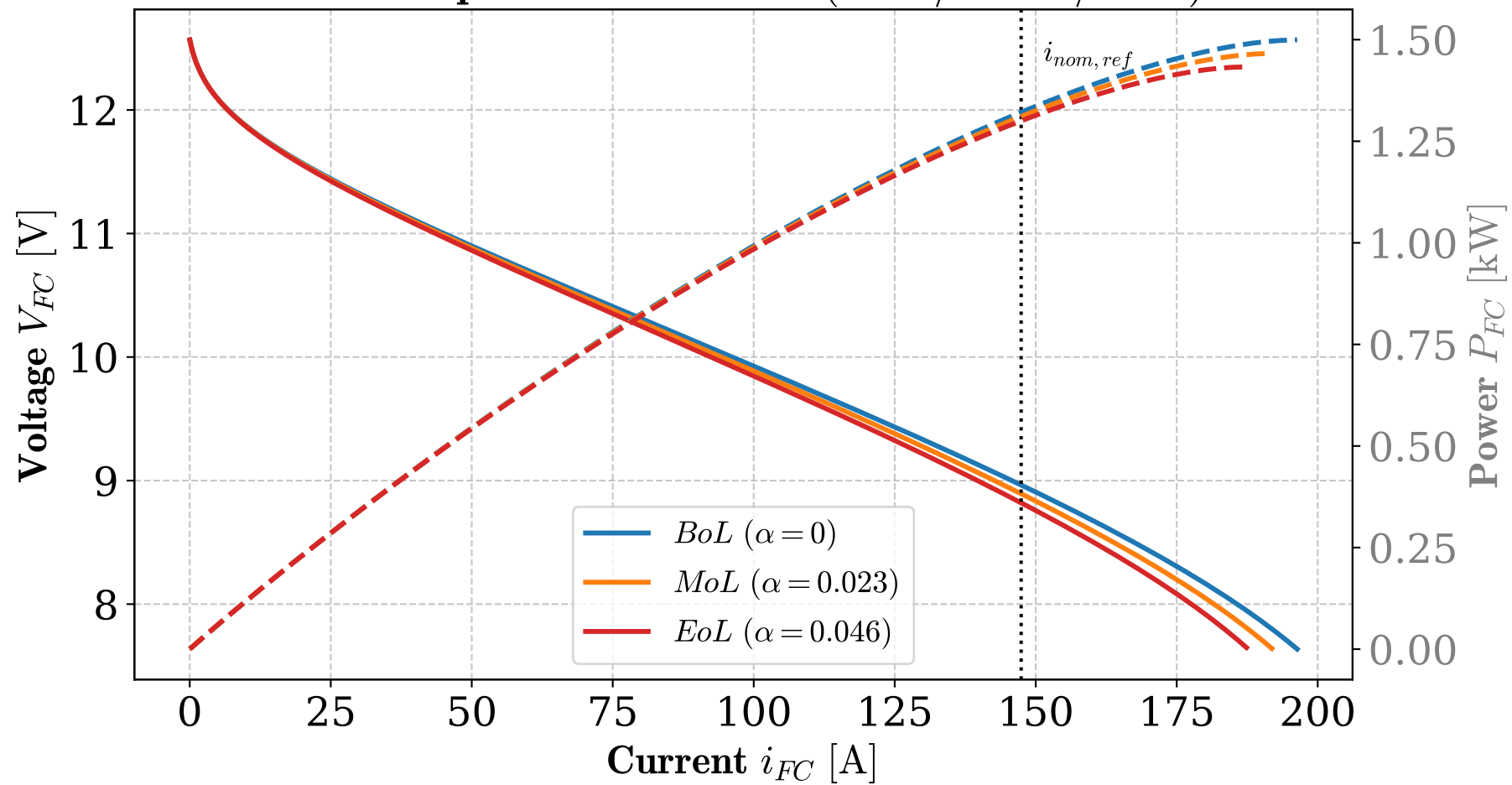
PEMFC polarization curve (BoL / MoL / EoL)
